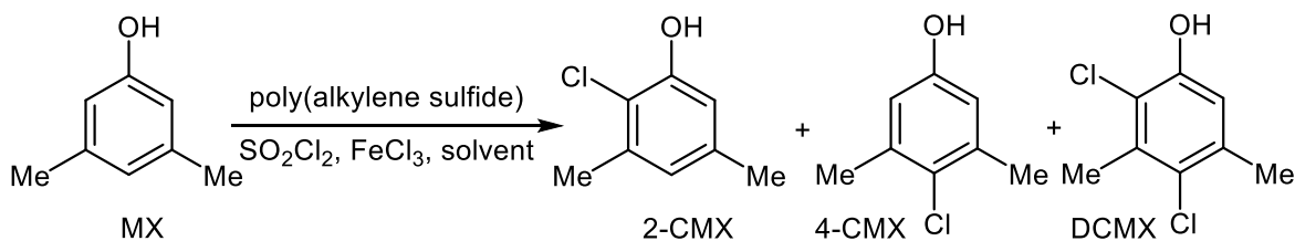
Scheme 3. Chlorination of m -xyleneol using sulfuryl chloride and poly(alkylene sulfide)s 1–26 .
