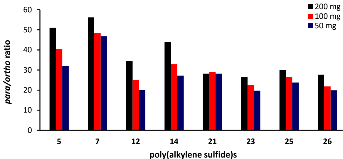
Figure 2. Effect of quantity of polymers on p/o ratio in chlorination of o -cresol.
