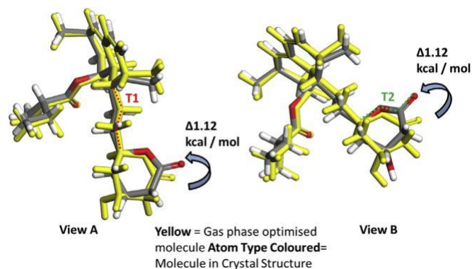
Figure 2. Conformational overlay of the gas phase-optimized lovastatin molecule and the molecule in the asymmetric unit of lovastatin.
