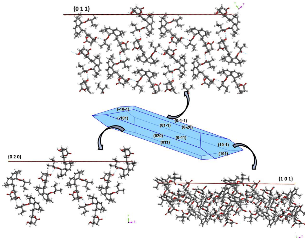
Figure 5. Attachment energy morphology of lovastatin together with the surface chemistry of the habit planes.
