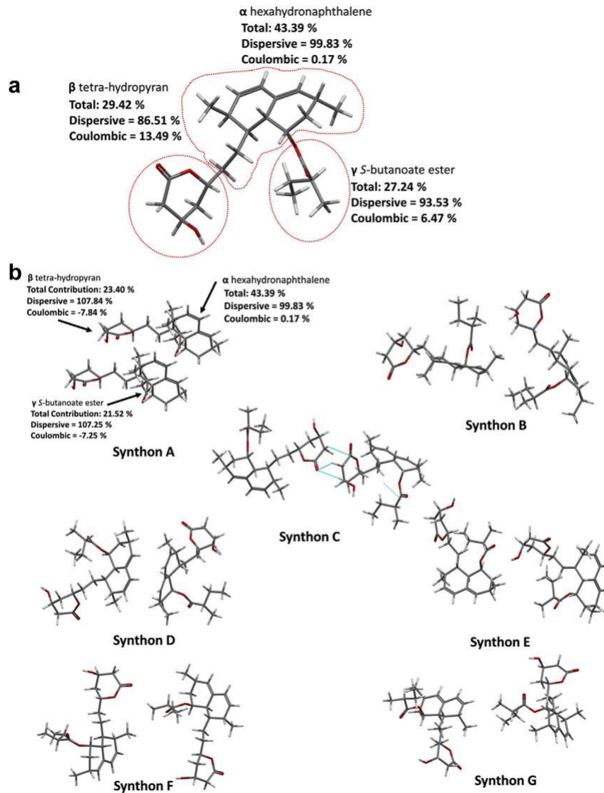
Figure 4. (a) The percentage contribution to the lattice energy provided by the 3 functional groups of the lovastatin asymmetric unit and the top 7 intermolecular synthons which contribute to the lattice energy of lovastatin.
