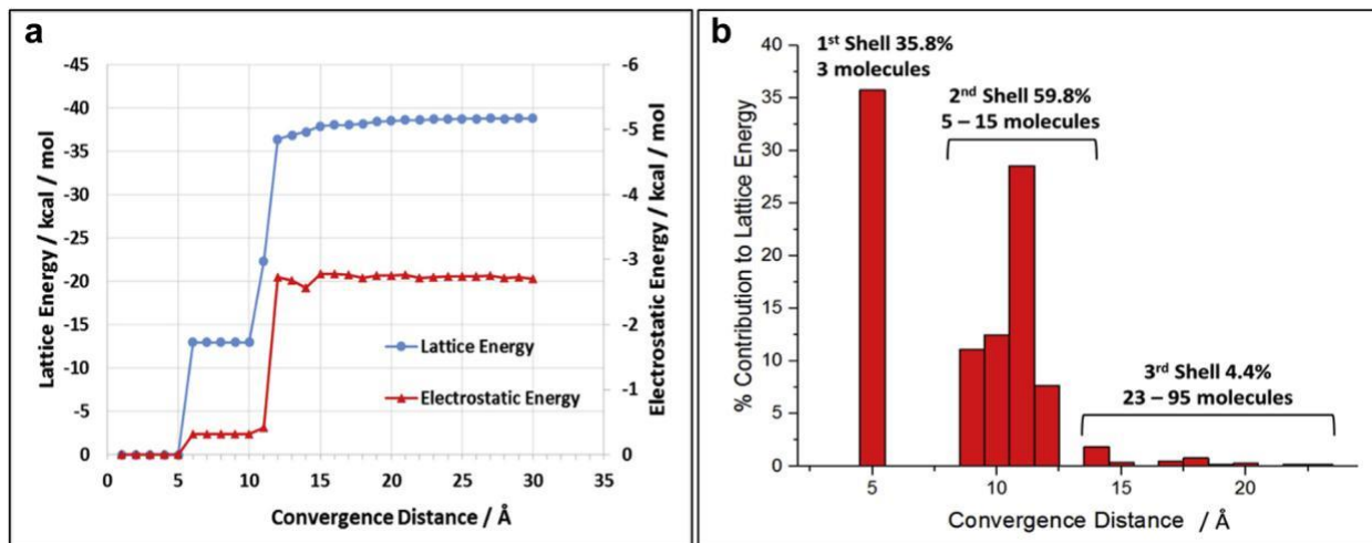
Figure 3. Convergence of the calculated lattice total energy and the % contribution to the lattice energy.
