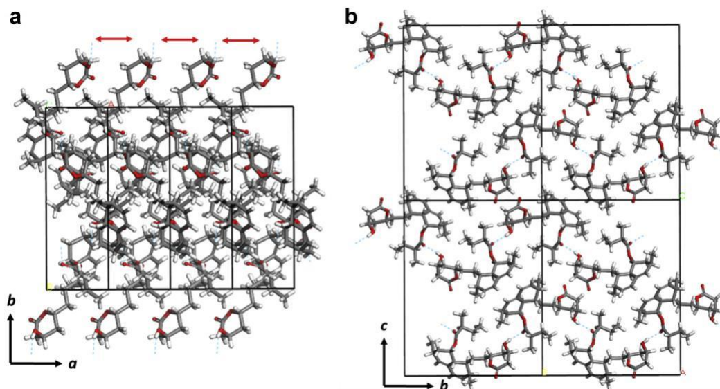
Figure 1. The crystal structure of lovastatin viewed down the a and c axes.
