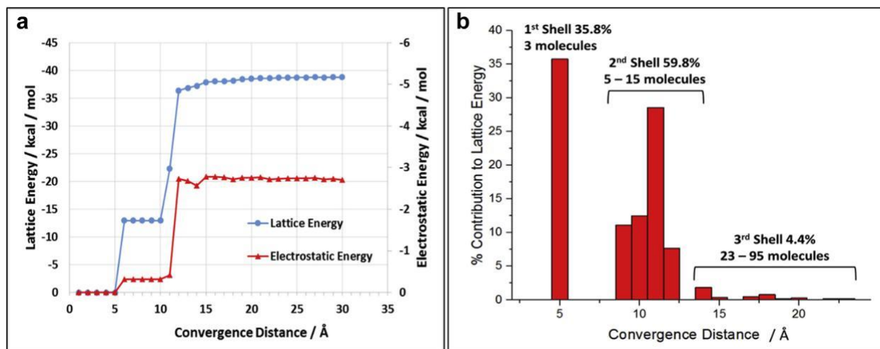
Figure 3. Convergence of the calculated lattice total energy and the % contribution to the lattice energy.
