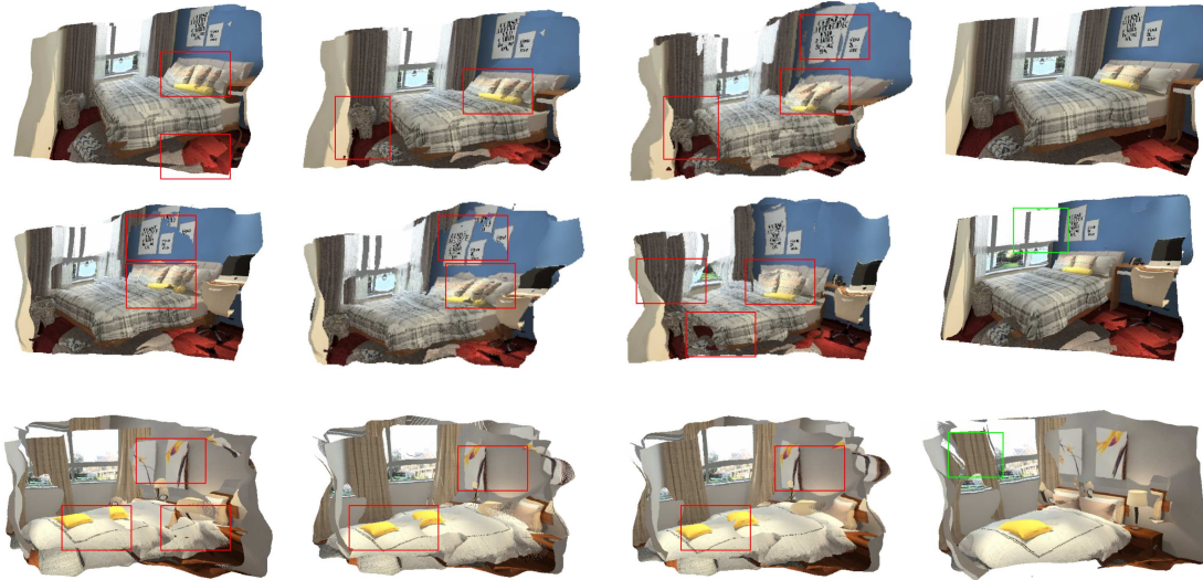
Figure 5. Comparison of different alignment methods: From left to right are results of standard ICP algorithm [31], 4PCS [40], global alignment using the estimated depth without the help of semantic branch, and our joint global and local alignment method.
