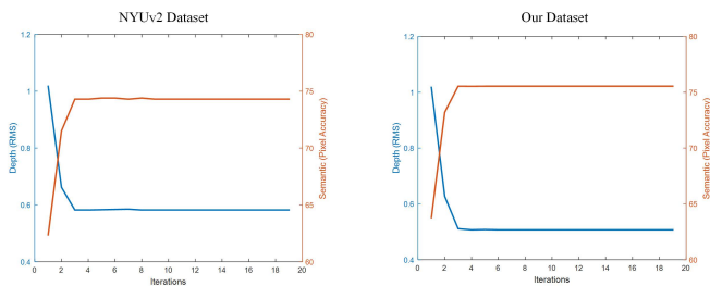
Figure 6. Convergence curves of the proposed IterNet for NYUv2 dataset [5] and our dataset (averaged over all test images in each dataset).
