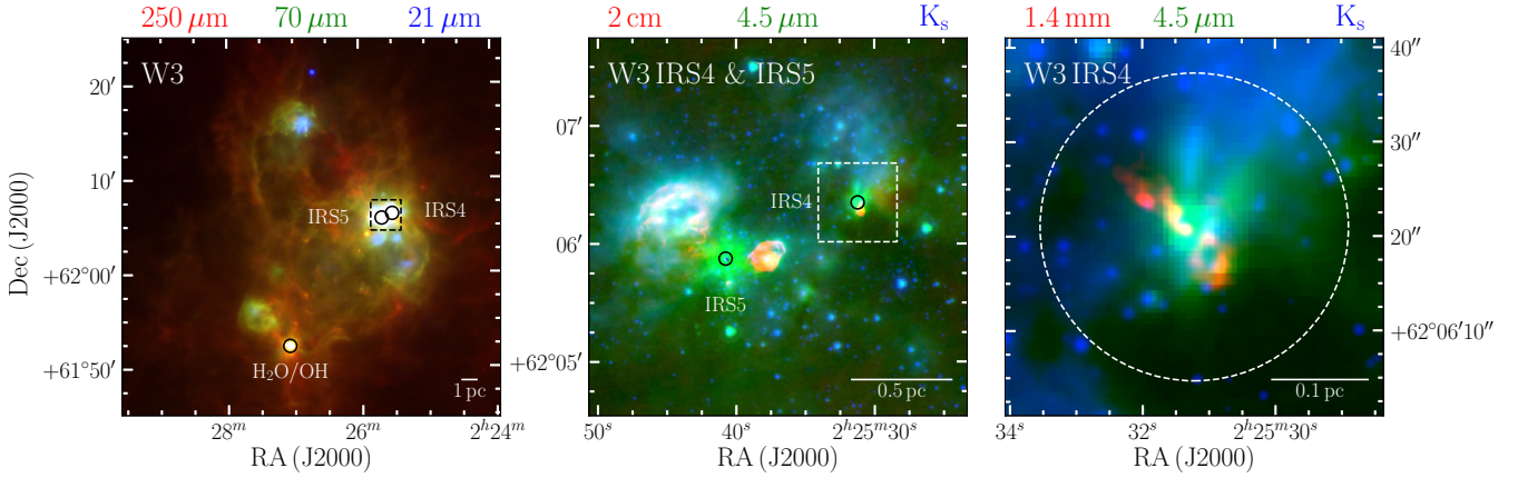
Fig. 1. Overview of the W3 star formation region showing the larger-scale context of W3 IRS4. Left: infrared three-colour image of W, where red is Herschel Hi-GAL (Molinari et al. 2016) 250 \mu\text{m} , green is Hi-GAL 70 \mu\text{m} , and blue is MSX 21 \mu\text{m} (Price et al. 2001). The three brightest far-IR sources, W3 OH/H 2 O, W3 IRS4, and W3 IRS5, are indicated with black circles. The region for the middle panel is indicated with a black dashed box. Middle: three-colour image of W3 IRS4 and IRS5, where red is 14.9 GHz radio free-free continuum from Tieftrunk et al. (1997) to emphasise ionised gas, green is Spitzer IRAC 4.5 \mu\text{m} (Ruch et al. 2007), and blue is Large Binocular Telescope (LBT, Hill et al. 2006) K_s data from Bik et al. (2012). The locations of W3 IRS4 and IRS5 are indicated with black circles, with the white dashed box indicating the region covered in the left-hand panel. Right: three-colour image focusing on W3 IRS4, where red is the NOEMA 1.4 mm continuum presented in this paper, imaged with natural weighting, while green and red are as in the middle panel. The dashed white circle shows the full-width half-maximum of the primary beam for the NOEMA continuum observations.
