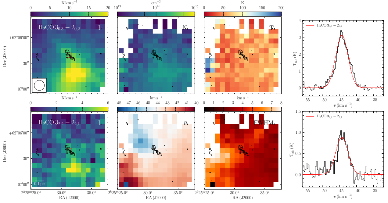
Fig. C.1. XCLASS fitting for the IRAM 30 m \text{H}_2\text{CO} data. The panels show: integrated intensity (between -87.5 and 2.2 km s ^{-1} ) in the \text{H}_2\text{CO} 3_{0,3}-2_{0,2} (top-left) and 3_{2,2}-2_{2,1} (bottom-left) transitions; column density in p- \text{H}_2\text{CO} (top-middle-left); excitation temperature (top-middle-right); peak velocity (bottom-middle-left); FWHM (bottom-middle-right); example spectra (black) and XCLASS model fits (red) for \text{H}_2\text{CO} 3_{0,3}-2_{0,2} (top-right) and 3_{2,2}-2_{2,1} (bottom-right). The beam is shown in the top-left panel. The black contours in the maps show the NOEMA 1.4 mm continuum smoothed to a FWHM of 0.8'' , as used for the analysis of the combined \text{H}_2\text{CO} data in Sect. 3.2, starting at 5\sigma and increasing to 45\sigma in 10\sigma steps. The spectra are extracted at the position covering the hot-core, which is indicated in the right-hand panels with a red square. A scale-bar is shown in the lower-left panel.
