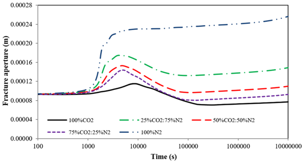
FIGURE 16 Time evolution of the fracture aperture at measuring point A for the case of different CO 2 /N 2 injection compositions [Colour figure can be viewed at wileyonlinelibrary.com ]
