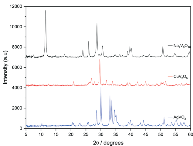
Fig. 1 XRD patterns for synthesised bronzes: Na 2 V 6 O 15 (black), CuV 2 O 5 (red), AgVO 3 (blue).
