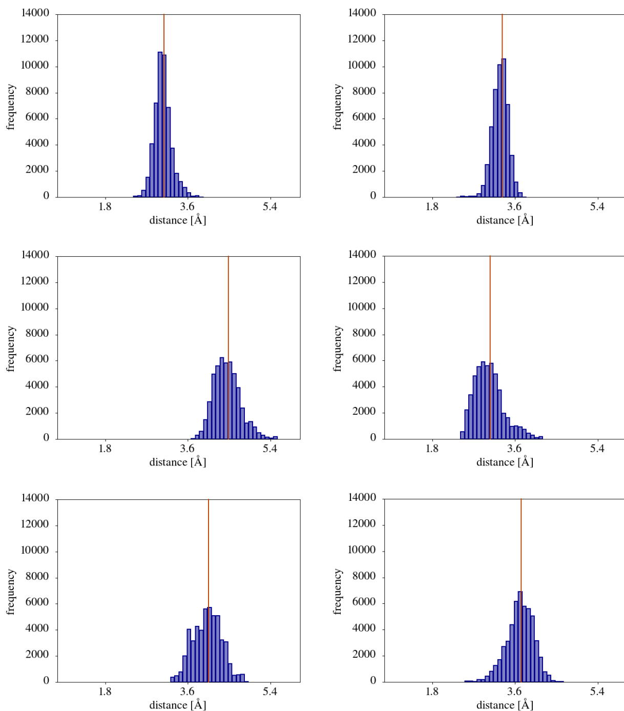
Figure 5. Histogram, during a 50 ps simulation at 300 K, of the distance between the centre of the methanol cluster ( M ) adsorbed at the T12 site and the centre of the exposed T12 acid site ( A ). Models are considered having one (left column) and two (right column) acid sites, with one (top row), three (middle row) and five (bottom row) methanol molecules per unit cell. An orange vertical line highlights the average distance.
