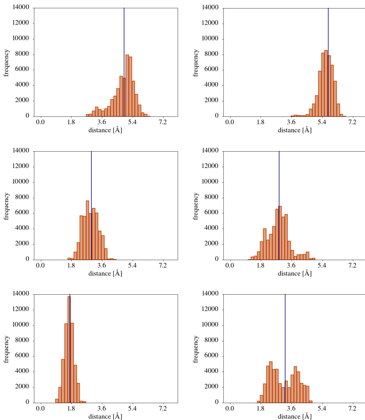
Figure 6. Histogram, during 50 ps simulation at 300K, of the distance between the geometric centre for the methanol cluster ( M ) adsorbed at the T12 site and the centre of the zeolite pore ( R ). Models are considered having one (left column) and two (right column) acid sites, with one (top row), three (middle row) and five (bottom row) methanol molecules per unit cell. A dark-blue vertical line highlights the average distance.
