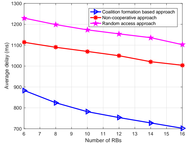
Fig. 6. Network average delay vs. number of RBs ( M = 30, K = 6 ).
