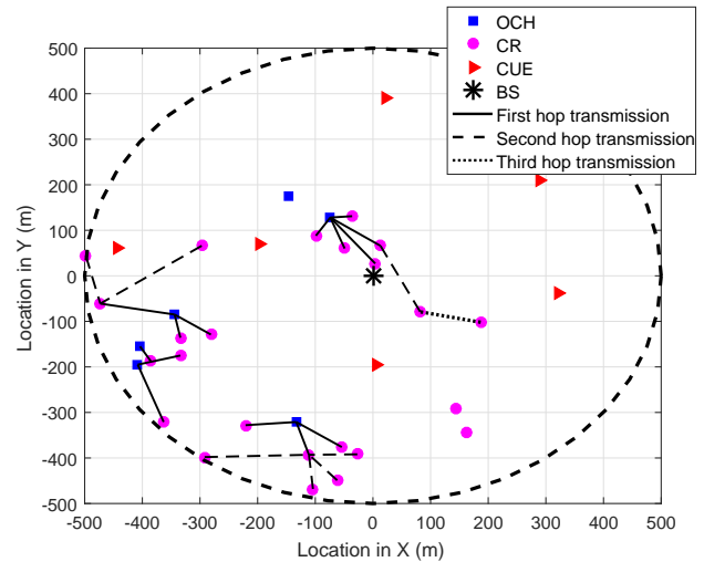
Fig. 3. An illustration of user locations and multihop D2D transmissions with K OCHs, (M - K) CRs and C CUEs ( M = 30, K = 6, C = 6 ).
