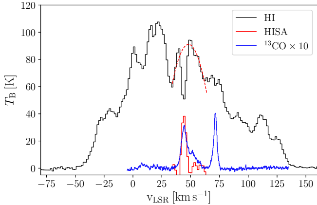
Fig. 2. H I, HISA, and ^{13}\text{CO} spectra. The black curve shows an example spectrum of H I emission ( T_{\text{on}} ) from -80 to 160 \text{ km s}^{-1} averaged over an area of 180'' \times 180'' centered in \ell = 19.9^\circ , b = -0.5^\circ . The dashed red curve is a second-order polynomial fit ( T_{\text{off}} ) to the absorption-free channels of the H I spectrum at 33.5\text{--}43.0 and 56.0\text{--}65.5 \text{ km s}^{-1} (see Sect. 2.2). We estimated the HISA spectrum by then subtracting the H I spectra from the fitted background emission. The GRS ^{13}\text{CO} spectrum (Jackson et al. 2006) covering velocities from -5 to 135 \text{ km s}^{-1} is shown in blue and has been multiplied by a factor of ten for better visibility.
