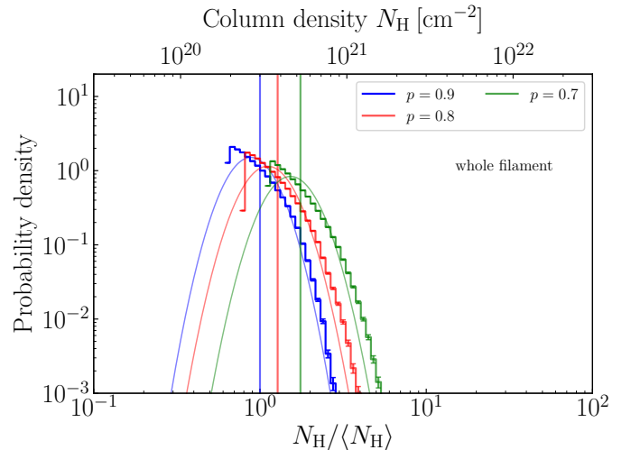
Fig. A.2. H I self-absorption N-PDFs for different values of background fraction p . The plot shows the derived N-PDF of the whole filament marked by both the red polygons in Fig. 11. The blue, red, and green distributions correspond to a background fraction of 0.9, 0.8, and 0.7, respectively. The vertical lines show the corresponding mean column densities.
