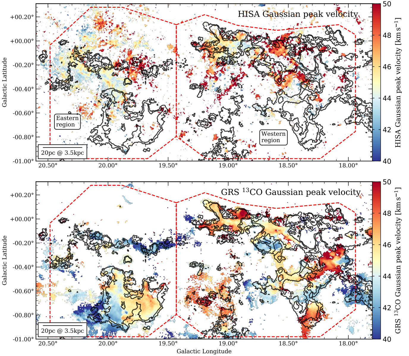
Fig. 6. Peak velocity maps. Upper panel: HISA peak velocities inferred from Gaussian fits. Lower panel: fitted ^{13}\text{CO} peak velocities. The black contours indicate the integrated ^{13}\text{CO} emission at levels of 10.5 and 15 \text{K km s}^{-1} for reference. The red dashed polygons mark the eastern and western part of the filament that were used for a separate analysis.
