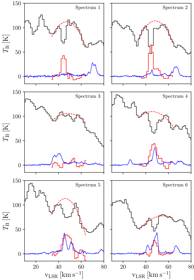
Fig. 4. HI ( T_{\text{on}} ) and extracted HISA spectra ( T_{\text{off}} - T_{\text{on}} ) toward the regions marked by the yellow circles in the bottom panel of Fig. 1. The colors are the same as described in Fig. 2.
