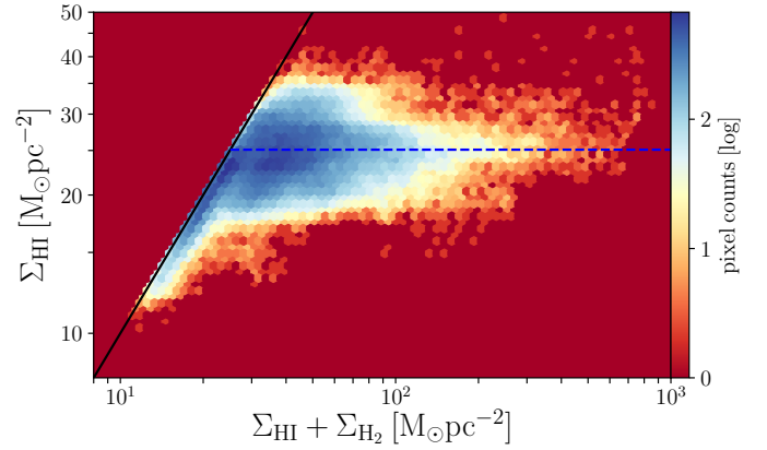
Fig. 15. H I-to-H 2 transition. The plot shows the H I mass surface density traced by H I emission as a function of the total hydrogen mass surface density. The black solid line indicates a 1-to-1 relation. The dashed blue line shows a fit to the mean of the distribution.
