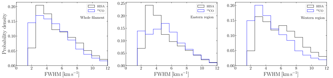
Fig. 9. Histogram of line widths. The histograms show the line widths of HISA and ^{13}\text{CO} in black and blue, respectively. Middle and right panels: line width distribution in the regions marked by the left and right polygon in Fig. 8, respectively.
