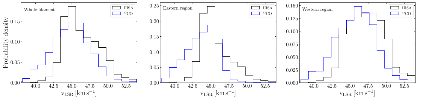
Fig. 7. Histogram of peak velocities. The histograms show the peak velocities of HISA and ^{13}\text{CO} in black and blue, respectively. Middle and right panels: velocity distribution in the regions marked by the left and right polygon in Fig. 6, respectively.
