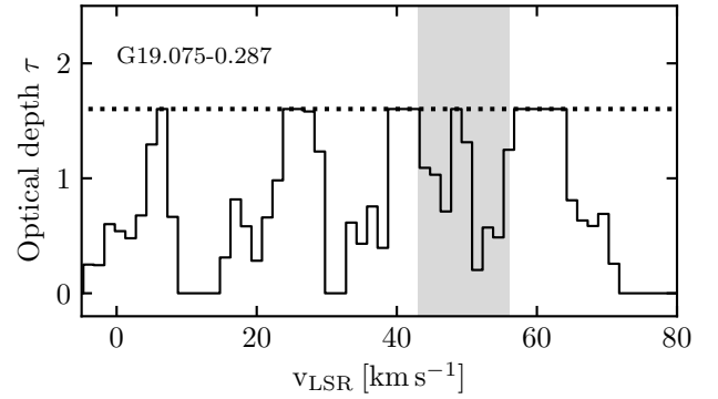
Fig. 12. Optical depth measurement toward the H II region G19.075-0.287 (Wang et al. 2018). The plot shows the optical depth as a function of LSR velocity and was computed using Eq. (9). For some channels, the absorption spectrum saturates and the measured optical depth is a lower limit of \tau = 1.6 , which is indicated by the horizontal dotted line. The gray shaded area indicates the velocity range between 43 and 56 \text{ km s}^{-1} , where HISA features have been extracted.
