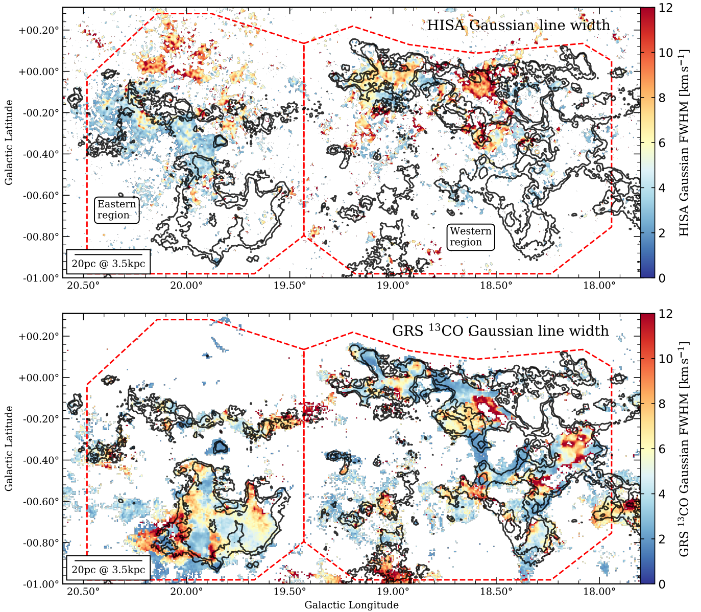
Fig. 8. Line width maps. Upper panel: HISA line widths inferred from Gaussian fits. Lower panel: fitted ^{13}\text{CO} line widths. The black contours indicate the integrated ^{13}\text{CO} emission at levels of 10.5 and 15 \text{K km s}^{-1} for reference. The red dashed polygons mark the eastern and western part of the filament that were used for a separate analysis.
