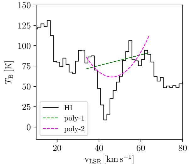
Fig. 3. Comparison of baseline fits toward continuum emission. The black curve shows an example spectrum of H I emission centered in \ell = 18.95^\circ , b = -0.03^\circ that is contaminated by continuum emission. The dashed magenta and green curve show a second and first order polynomial fit to the velocity channels of the H I spectrum at 33.5\text{--}43.0 and 56.0\text{--}65.5 \text{ km s}^{-1} , respectively. Due to the continuum contamination, the second order polynomial yields a bad fit to the HISA baseline.
