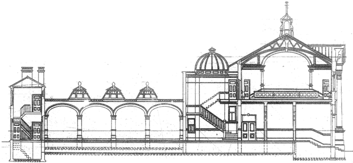
Figure 5. West Bromwich Library, Stephen J Holliday 1907 Long section. Schofield, H. Borough Engineer and Surveyor, 1949. Courtesy Sandwell Metropolitan Borough Council Architect's Unit
