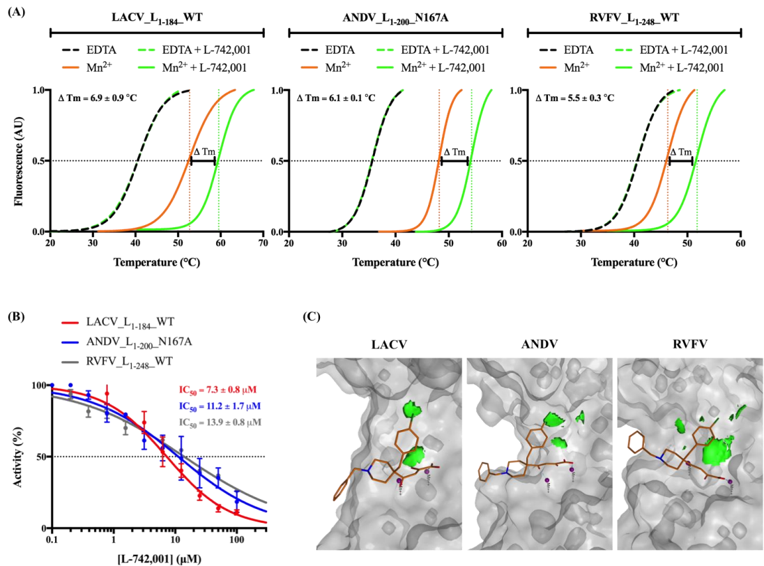
Fig. 2. L-742,001 inhibitory molecular interactions with Bunyavirales Cap-ENDO's.
