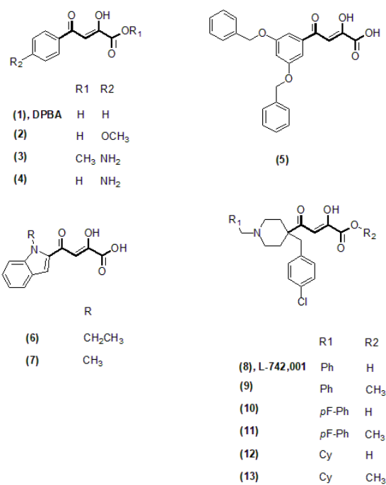
Fig. 1. Schematic representation of compounds (1)-(13); in bold the chelating region.
