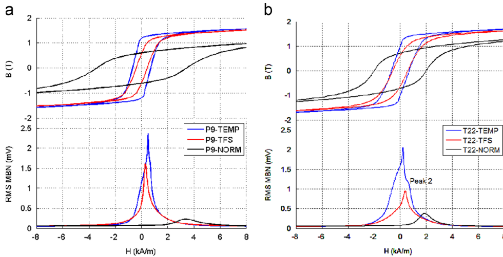
Fig. 3. B - H loops and corresponding MBN profiles for (a) P9 samples, (b) T22 samples.
