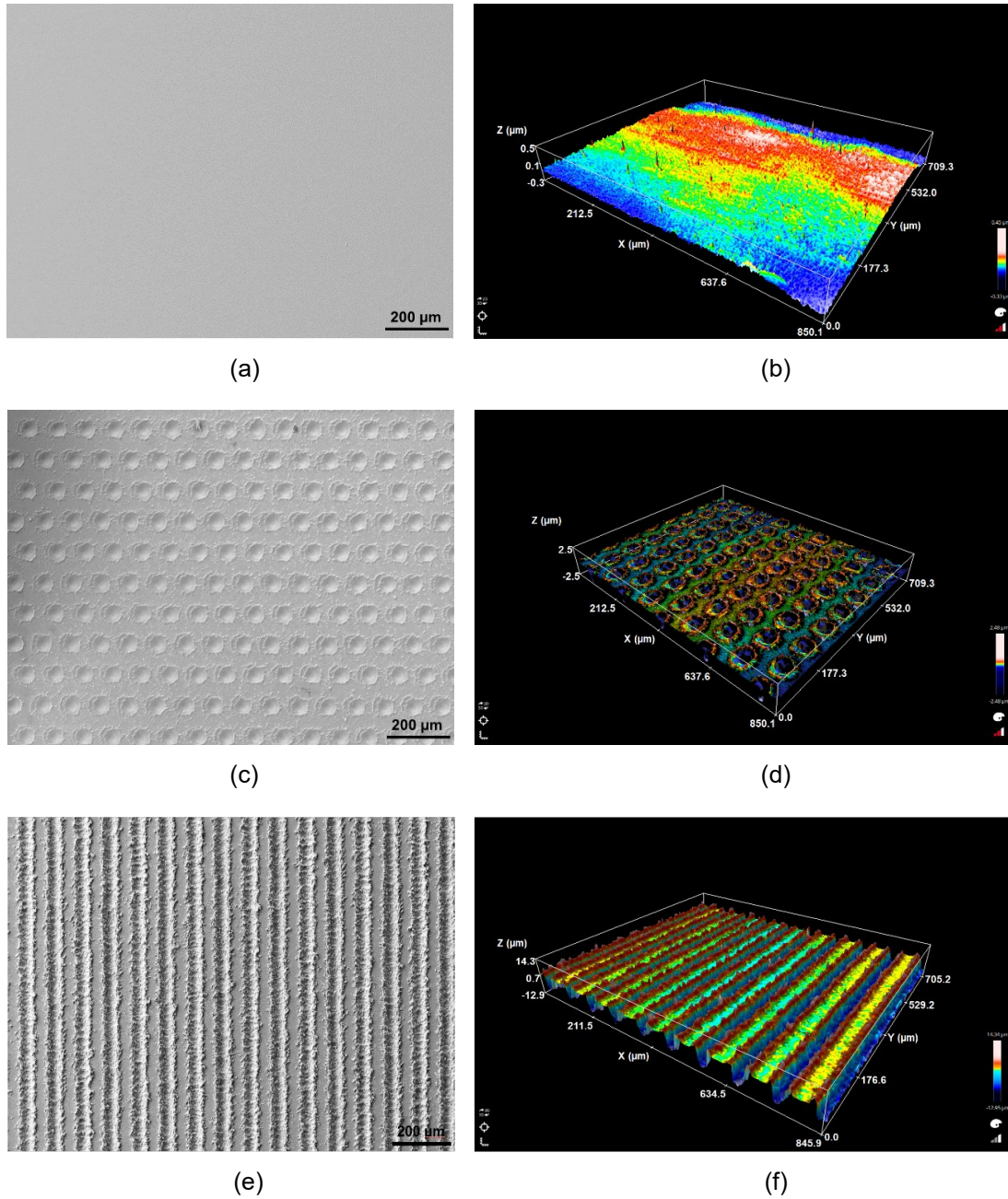
Fig. 2. SEM images of Vitreloy 105 surfaces (a, c, e) and their corresponding 3D topography (b, d, f). (a)(b) for the as-cast, (c)(d) for the dimple textured and (e)(f) for the groove textured sample.
