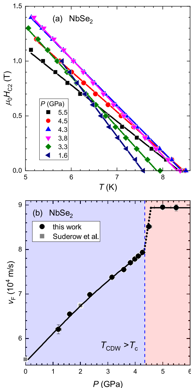
FIG. 4. Upper critical field and Fermi velocity in 2H\text{-NbSe}_2 . (a) Linear fits to H_{c2}(T) have been used to extract v_F(P) shown in (b). For details see S III of the Supplemental Material Ref. [26]. Data of Suderow et al. [23] have been included in (b) for the pressure range with good agreement of T_c (see SII of the Supplemental Material Ref. [26]). Lines are guides to the eye.
