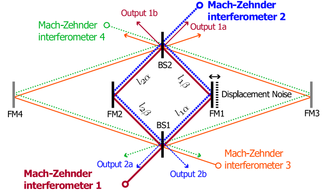
FIG. 1 (color online). Schematic of one possible 2D optical configuration of a displacement-noise-free interferometer. Light beams which follow common paths (thick, thin) travel in opposite directions, and the four MZIs share the two beam splitters (BS1 and BS2). The motion of each folding mirror (FM) is sensed by two MZIs, and the motion of the beam splitters is sensed by all four MZIs.
