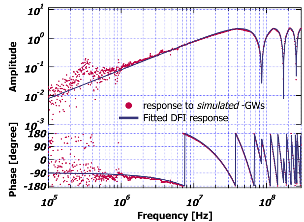
FIG. 5 (color online). The effects of the response functions of EOMs and HPDs on the DFI signal (solid-green curve in Fig. 4) were compensated by using the response function to single detector, shown in red dots. This corresponds to an intrinsic DFI (bidirectional MZIs for this experiment) response function to a simulated GW signal. The solid curve is a fitted DFI response giving reasonable fitting parameters.
