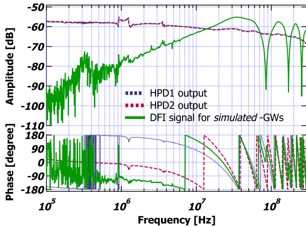
FIG. 4 (color online). The response functions from simulated -GW inputs to output signals. HPD1 and HPD2 response show almost the same response again in amplitude, whereas the phase delays in the higher frequency band are essentially different from that of displacement noise, which is the very reason why the summed signal (DFI signal) remains GW sensitive as is shown in the solid-green curve.
