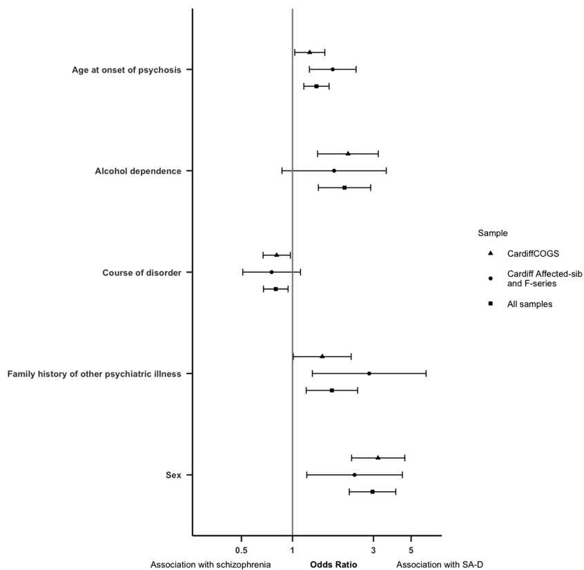
Fig. 2. Odds ratios (OR) and confidence interval for each lifetime clinical characteristic included in the replication and meta-analysis, analyzed in the CardiffCOGS sample, the replication samples, or in the meta-analysis of all samples. OR > 1 indicates association with SA-D; OR < 1 indicates association with schizophrenia.
