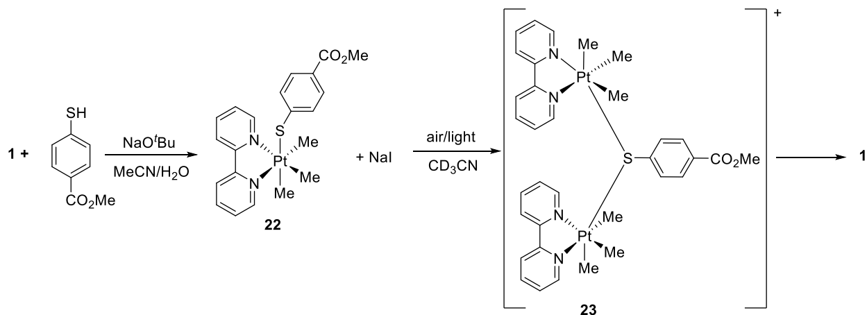
Scheme 6: Decomposition of 22 .
