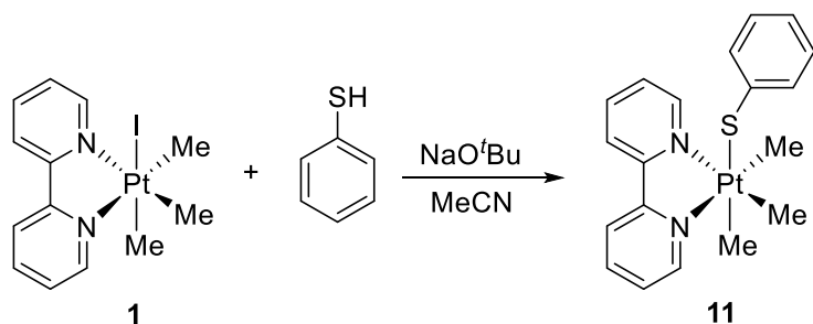
Scheme 4. Synthesis of \text{Me}_3\text{bpyPtSPh} 11
