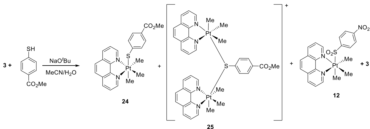
Scheme 6: Decomposition of 22 .
