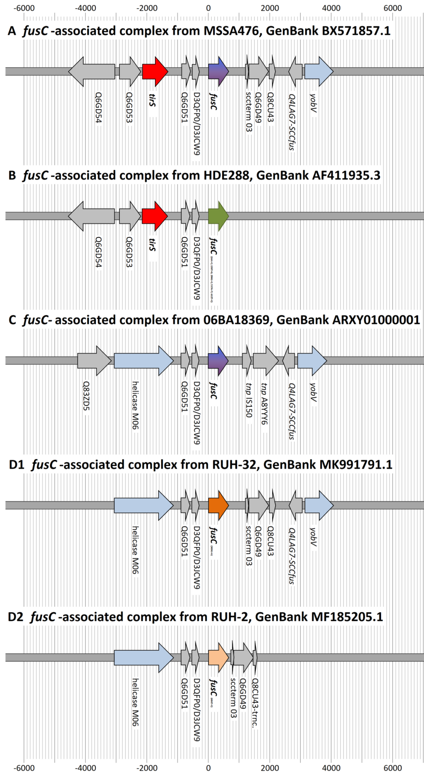
Figure 2. The different sets of genes directly accompanying fusC in M58 and in previously published SCCfus or SCCmec/fus elements.
