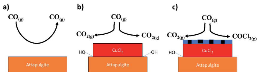
Fig. 17 Schematic representation of processes associated with the reactions described in Section 3.1. (a) CO exposure over the support material at elevated temperatures – no significant degree of reaction (Fig. 11); (b) CO exposure to supported \text{CuCl}_2 at elevated temperature and in the absence of a chlorine pre-treatment – \text{CO}_2 formation is exclusively observed that is thought to occur via a reaction with hydroxyl groups present at the \text{CuCl}_2 /support interface (Fig. 9(a)); (c) CO exposure to a chlorine pre-treated supported \text{CuCl}_2 catalyst at elevated temperature – CO oxidation pathway is inhibited due to displacement of interfacial hydroxyl groups by the chlorine, whilst the chlorine pathway is activated by the presence of copper chloride surface defect sites (Fig. 9(b)). The chlorine defect sites are schematically indicated in (c) by the thin blue hatched area at the surface of the \text{CuCl}_2 crystallite.
