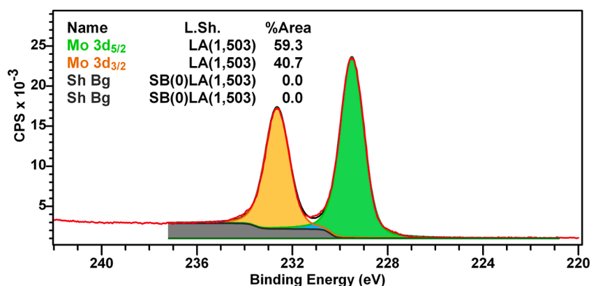
Fig. 2. Mo 3d doublet measured from molybdenum trioxide at a point on the sample where there was no evidence of sulfur. A component used in a peak model to accommodate a Shirley background shape is constructed from the bell-shaped line-shape LA(1,503) by applying a prefix SB(0) to the line-shape LA(1,503).
