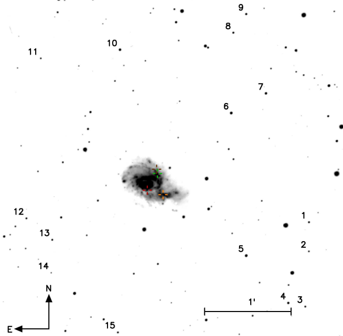
Fig. A.1. 4' \times 4' ePESSTO NTT+EFOSC2 r -band image of the field of NGC 3256 on 2018 January 16. The locations of sequence stars, SN 2018ec (green), AT 2018cux (red), PSN102750 (brown), and SN 2001db (orange) are indicated. North is up, east is left.
