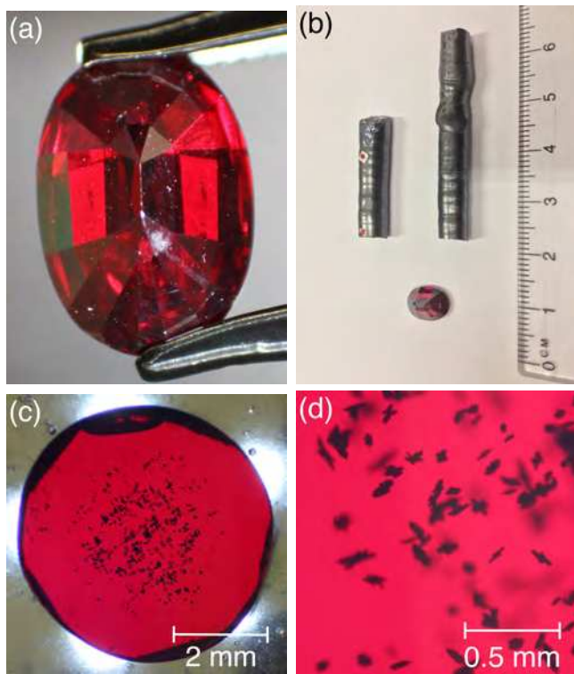
FIG. 1. (a) A commercially available natural cuprite gemstone. (b) Two synthetic single crystals of \text{Cu}_2\text{O} grown in this work with the same natural gemstone for scale. (c) Backlit slice of optically polished synthetic crystal. (d) Higher magnification optical image of the same slice highlighting the inclusions (dark specs).
