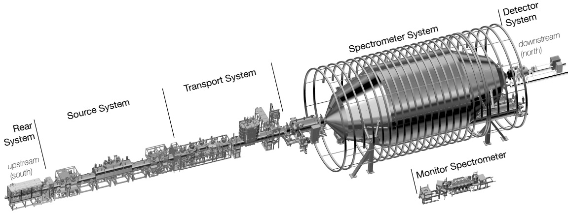
Figure 1. Schematic view of the KATRIN experimental setup. The overall length of the setup is about 70 m. The \beta -electrons from the tritium source are guided to the spectrometer by the electromagnetic field along the beamline. Electrons which have passed the spectrometer are then counted by the detector. Refer to section 7.6 for details about the Monitor Spectrometer (MoS) in its parallel beamline.
