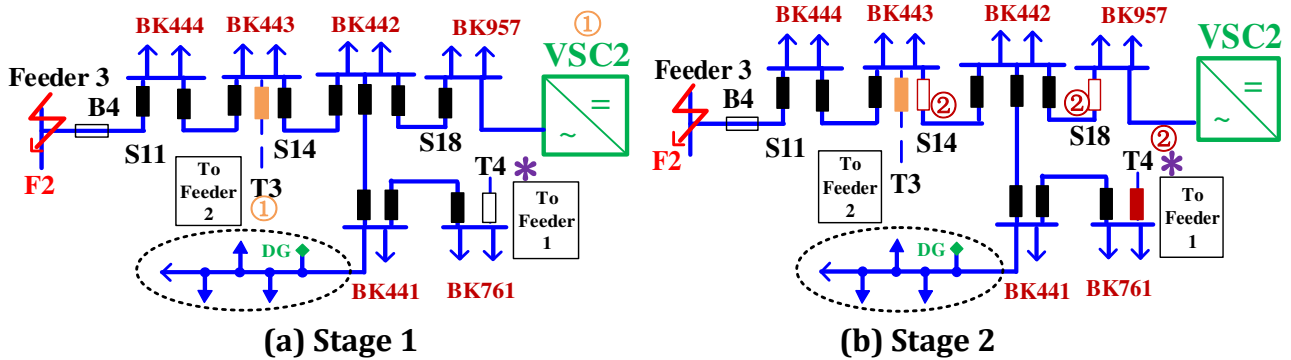
Fig. 11. Supply restoration stages in Scheme II under fault scenario F2.
