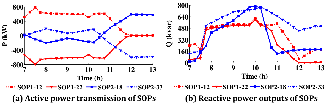
Fig. 8. Supply restoration strategies of SOPs in Scheme II.
