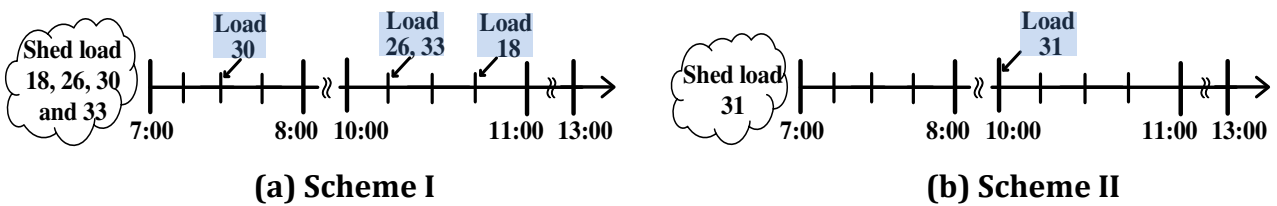
Fig. 6. Load pick-up schedule in the supply restoration period.
