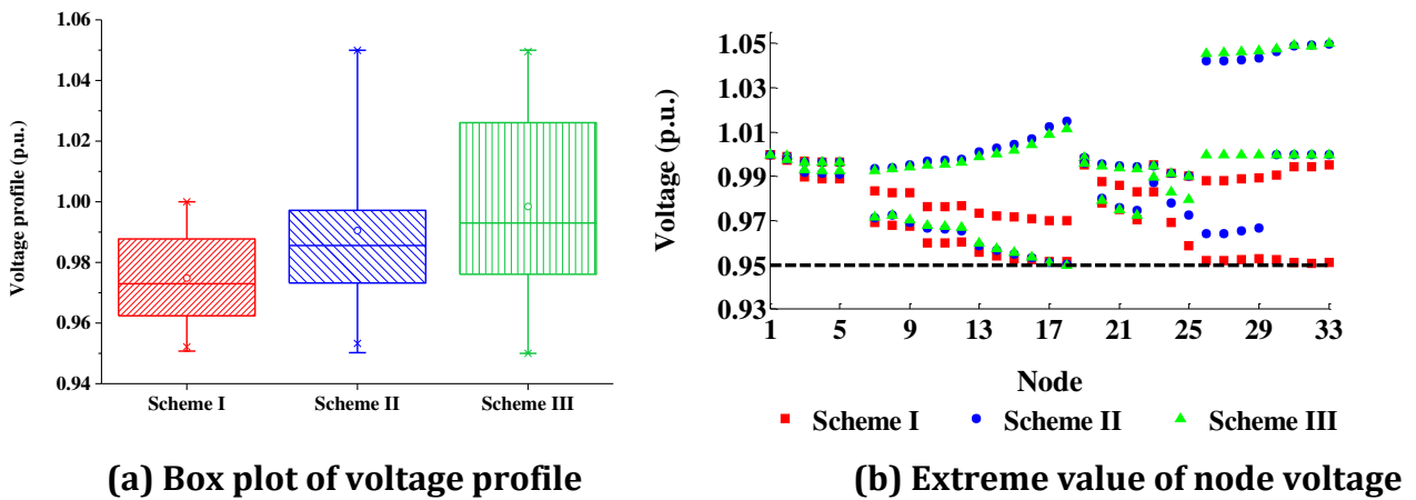
Fig. 7. Voltage profiles in Schemes I, II and III.
