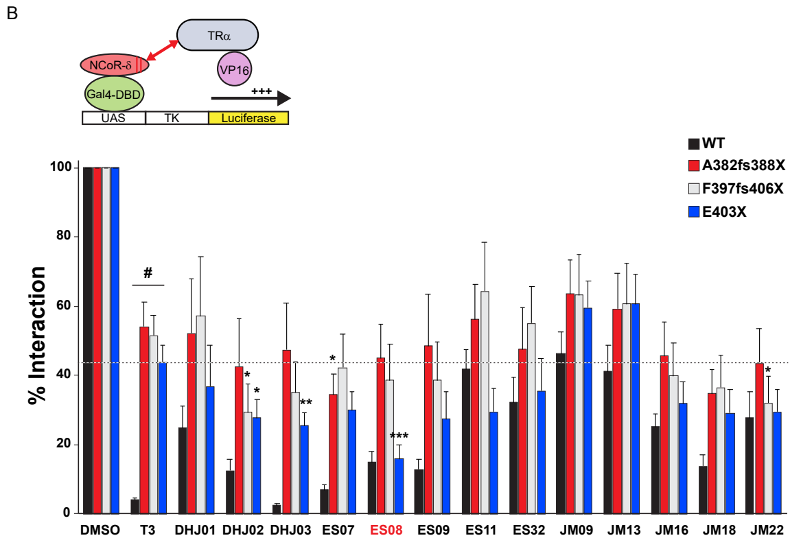
FIG 8 Interaction of VP16-TRα with GAL4-corepressor in mammalian cells. (A) Schematic representation of the cellular two-hybrid assay (left) and different human GAL4-corepressor isoforms (with locations of nuclear receptor interaction domains in red) tested (right). Below, this interaction of WT or mutant VP16-TRα fusions with different corepressor isoforms in the absence or presence of T3 is shown. Results are presented as mean ± SEM for at least 5 independent experiments performed in triplicate. *, P < 0.05 ; **, P < 0.01 ; ***, P < 0.001 for 0 nM T3 versus 10 nM T3 comparisons. (B) Interaction of GAL4-NCOR-δ with VP16-WT or mutant TRα fusions in the presence of vehicle (DMSO), 100 nM T3, or a different analogue. Results from at least 5 independent experiments are shown as percentages of interaction for WT or TRα mutants with NCOR-δ with vehicle. *, P < 0.05 ; **, P < 0.01 ; ***, P < 0.001 for comparisons of TRα mutants and T3 versus TRα mutants and analogue; # P < 0.001 for comparison of WT versus TRα mutants with 100-nM T3.
