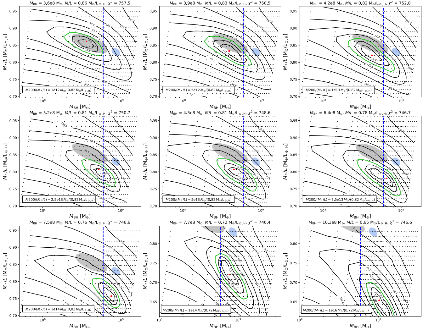
Figure D1. Results of our Schwarzschild run including a dark matter halo. In the runs, we have varied M_{\text{BH}} , M_{\text{*/}L} , and M_{200} . Each of the panels shows the M_{\text{BH}} - M_{\text{*/}L} grid (like Fig. 8) for an increasing dark matter fraction. While running Schwarzschild models, both M_{\text{BH}} and M_{200} need to be re-scaled for each model. The scale factor is the (M_{\text{*/}L}) of the grid divided by the starting (M_{\text{*/}L}) of the models. The confidence level was derived for each M_{\text{BH}} - M_{\text{*/}L} grid independently. As expected, with increasing dark matter fraction, the black hole mass increases and the M_{\text{*/}L} decreases. As expected, with increasing dark matter fraction, the black hole mass increases and the M/L decreases. Contrary to Fig. 8, here the M/L from JAM is larger or equal to that from Schwarzschild's models. This is because the former represents the total M/L , while the latter is that of the stellar component alone. When dark matter increases, the stellar M/L must decrease with respect to the total one, as observed.
