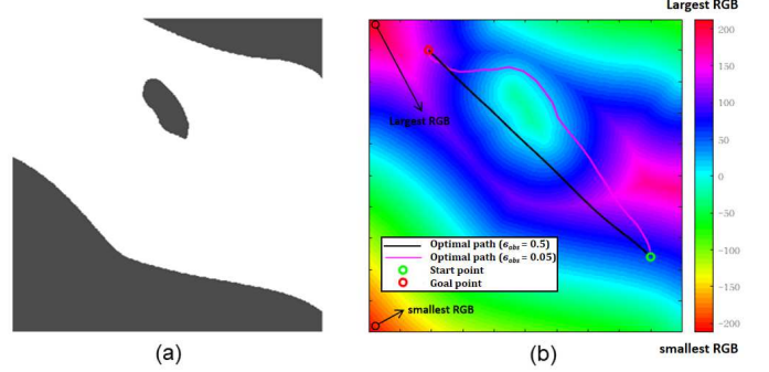
Fig. 3. Signed distance field of a coastal environment: (a) is the pixel map and (b) is the signed distance field of the map. In the signed distance field, the point with a larger RGB value is more secure than the point with a smaller RGB value. The value of \sigma_{obs} is inversely proportional to the weight of the behaviour (staying inside safe region). The point with a larger value on the color bar is relatively safe; on the other hand, the point with a smaller value on the color bar is relatively dangerous.
