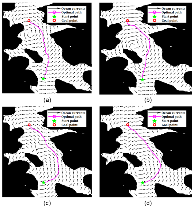
Fig. 16. Re-planning for static platform with time-varying ocean currents: From (a) to (d), the vortex moves from a position close to the platform start point to a position close to its platform goal point. In 10 repeated tests, the execution time of re-planning processes from (a) to (d) were 681.9 ms, 565.1 ms, 532.6 ms and 505 ms respectively.
