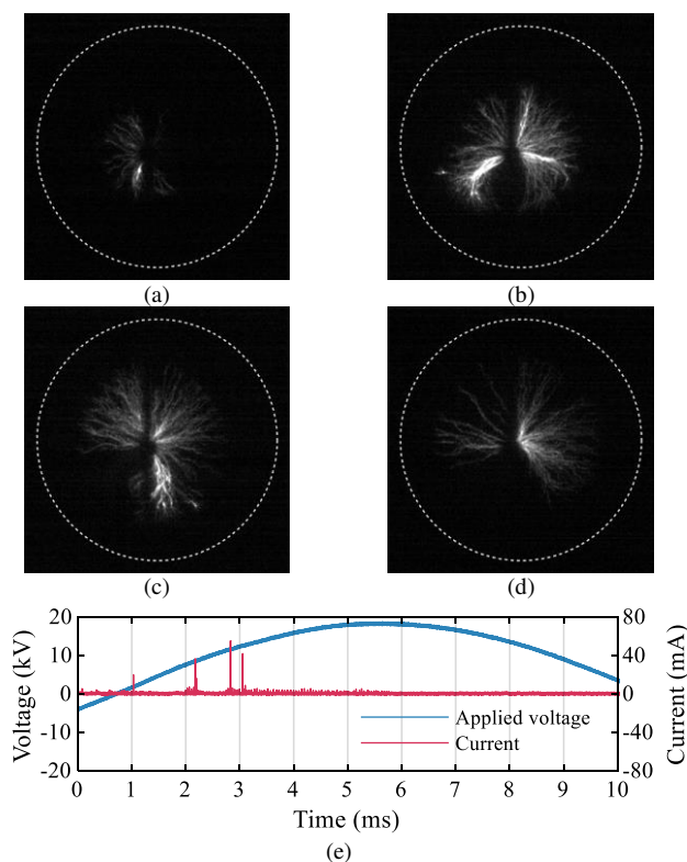
Fig. 7. Surface discharge development during the rising slope of the positive half-cycle of the applied AC voltage for the case of epoxy resin 4mm thickness in nitrogen (N 2 ) at 1 bar absolute pressure and rms applied voltage around 80% (13.13kV) of the corresponding rms FOV: (a) 1-2ms (b) 2-3ms (c) 3-4ms (d) 4-5ms and (e) voltage and current measurements.
