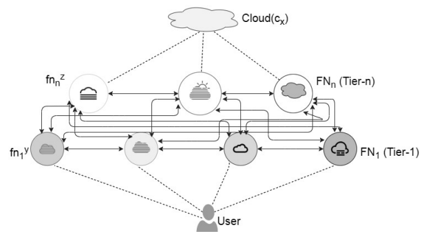
Fig. 1. Fog Architecture
