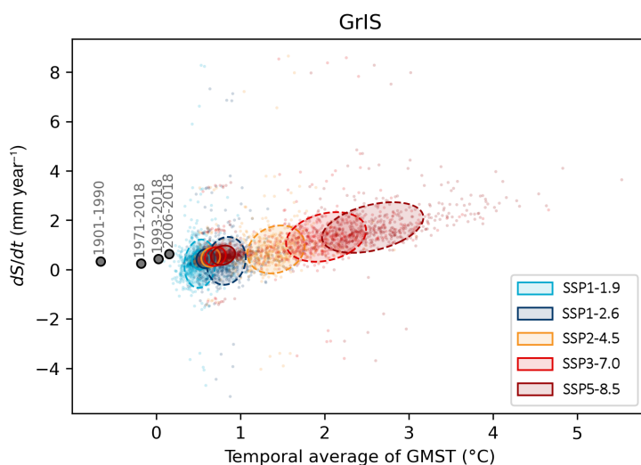
Figure 2. The transient sea level sensitivity (TSL) of the Greenland Ice Sheet (GrIS). The coloured dots show the sea level contribution of the ice sheet in \text{mm year}^{-1} for a given mean centennial temperature change based on CMIP6 Global Circulation Model forcing and temperature change for different Shared Socio-Economic Pathways (SSPs). Also shown as grey circles are observations and historical estimates of the ice sheet response. The x-axis shows the temporal average of global mean surface temperature (GMST). The y-label ( dS/dt ) is the change in mean global sea-surface height per unit time, in this case a year. It is apparent that over these timescales, the modelled response is a quasi-linear function of temperature.
