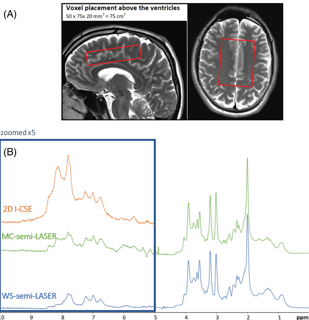
FIGURE 1 Illustration of VOI placement and spectral quality for a representative subject. A) The 75 cm 3 VOI placed centrally above the lateral ventricles with 5 mm spacing. B) Full spectra (downfield and upfield parts) for the semi-LASER-based techniques and the downfield part for frequency-selective 2D I-CSE documenting the overall spectral quality for all three techniques. When comparing noise levels, the differences in total number of scans and differences in different water-scaling have to be kept in mind (number of acquisitions and total scan times: 640, 768, 1280 and 32, 32, 55 min for 2D I-CSE, MC-semi-LASER, and WS-semi-LASER, respectively). I-CSE and MC-semi-LASER scaled with the water signal from MC-semi-LASER, WS-semi-LASER scaled by a reference signal recorded with the same sequence, but without VAPOR. Identical length of the acquired FID, no apodization, downfield part scaled by a factor of 5 compared to the upfield spectra)
