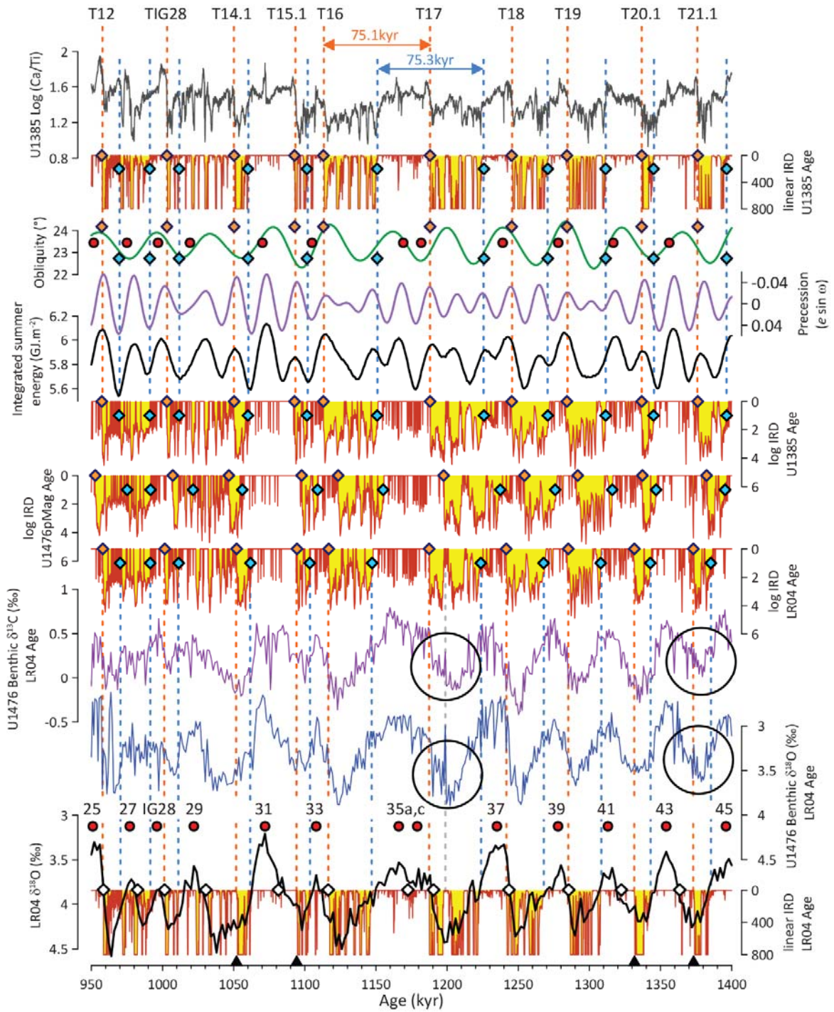
Figure 4. Obliquity loses grip on deglaciation. Throughout: red circles are interglacials (numbered; IG28 is a minimum in \delta^{18}O associated with MIS 28 (12)), white diamonds are deglacial transitions with respect
