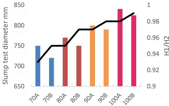
Figure 4. Diameters in slump tests and H_1/H_2 in L-box tests
