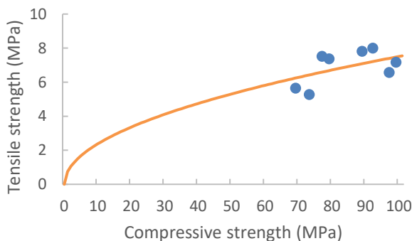
Figure 5. Relationship between splitting tensile strength and compressive strength of SCC mixes
