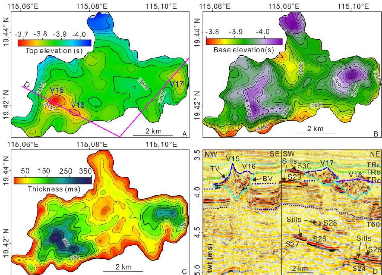
Figure 9: A: Morphology of the top surface of volcanoes V15, V16 and V17 in MZ1. B: Morphology of the basal surface of volcanoes V15, V16 and V17. C: Thickness of volcanoes V15, V16 and V17. D: Seismic profile showing the top (blue dashed lines) and base (cyan dashed lines) of volcanoes V15, V16, V17 and V18. Note that V18 is a slightly older than volcanoes V15-V17, though not shown in Figs. A-C. Horizons TRa, TRb, TRc, T60 and sills and high-amplitude, positive seismic reflections and cross-cutting the stratigraphic succession are marked in the figure.
