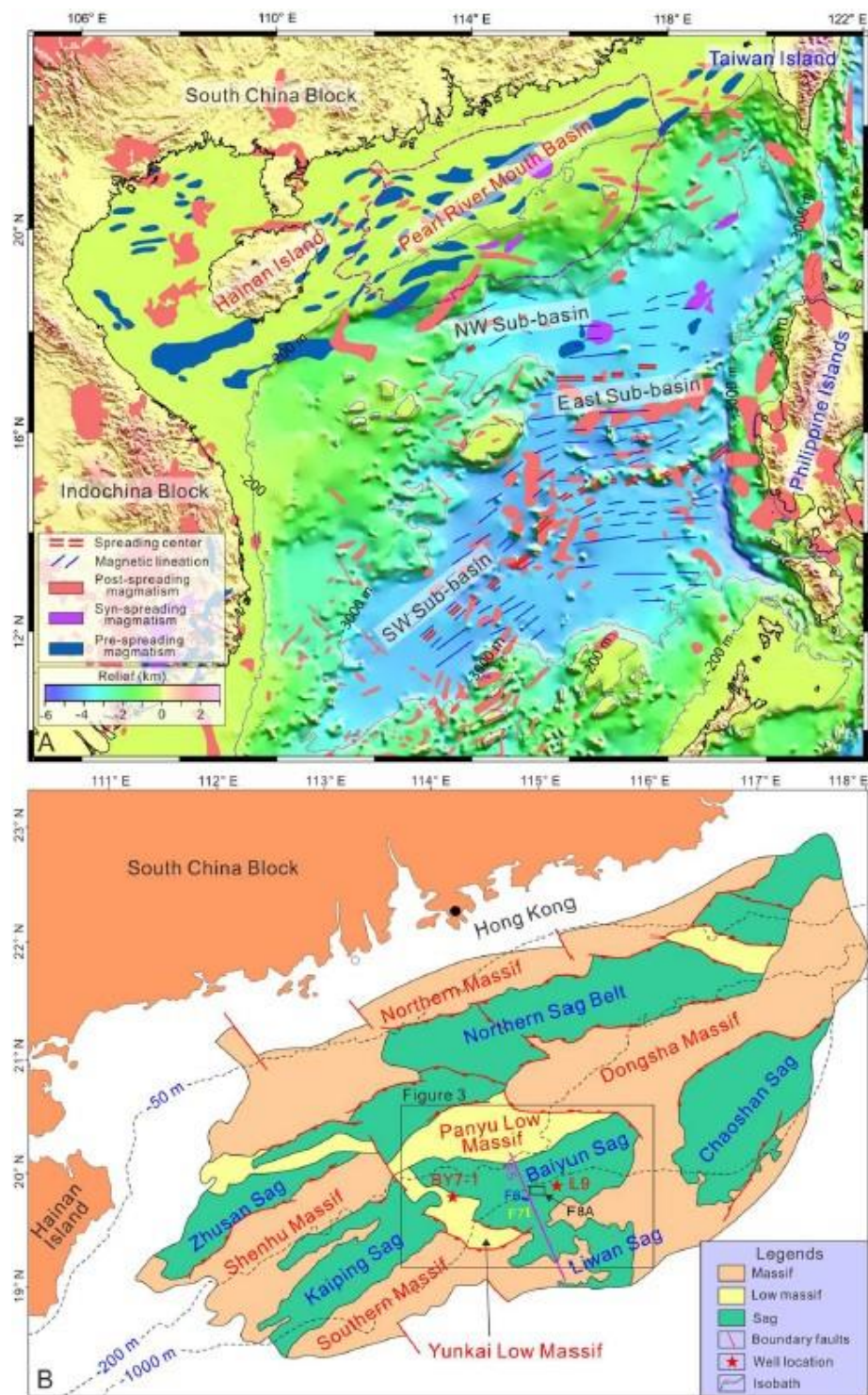
Figure 1. A: Geological setting of the northern South China Sea showing the Northwest (NW), East and Southwest (SW) sub-basins. The base map in this figure was re-drawn from He (2017). The locations of the spreading centre and magnetic lineations are from Briais et al. (1993) and Li et al. (2014). Pre-, syn- and post-spreading magmatism is modified from Hui et al. (2016); B: Geological subdivision of the Pearl River Mouth Basin. Wells BY7-1 and L9 are marked by red stars. The listric boundary faults (detachment faults) are modified from Pang et al. (2008) and Sun et al. (2014). This study is focused on the Baiyun Sag. F4-F7 indicate Figures 4 to 7.
