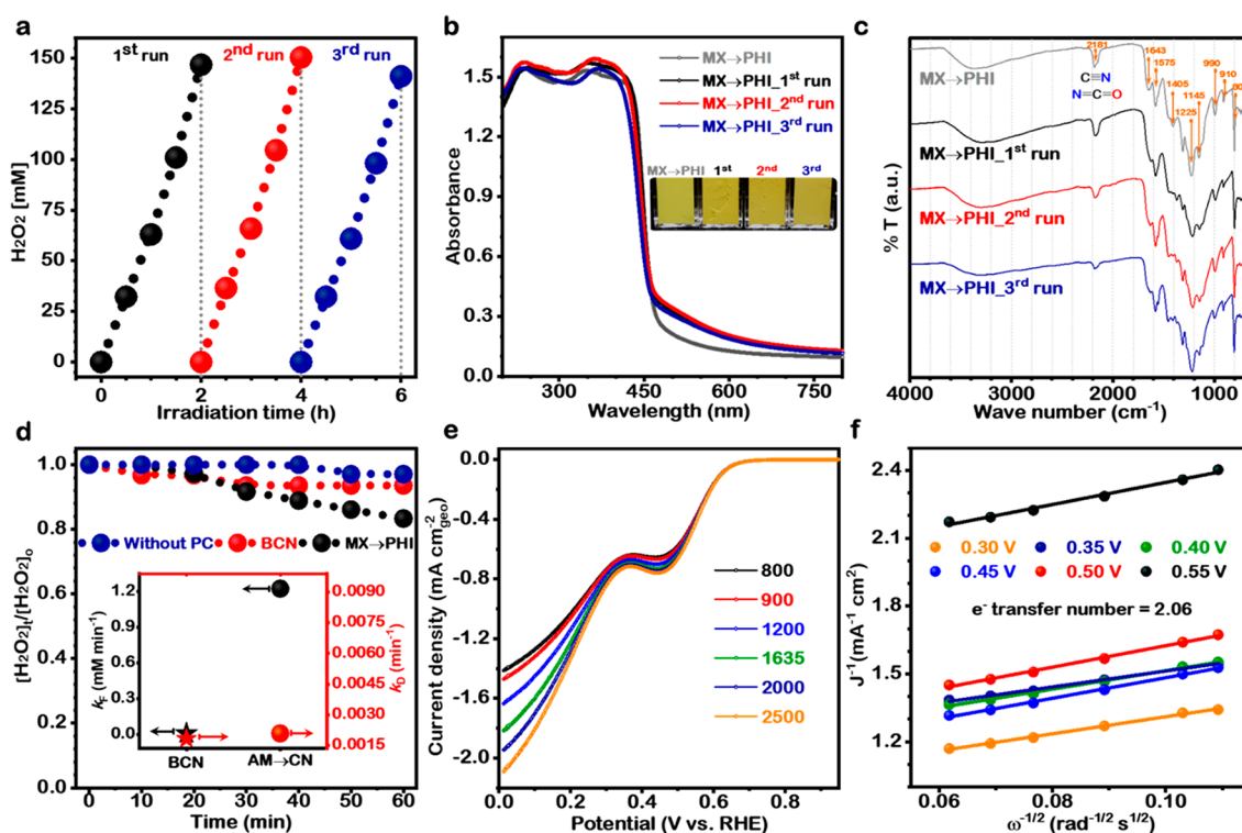
Figure 5. Stability, kinetics, and comparison. (a) Repeated run stability analysis of MX \rightarrow PHI to highlight the recyclability. (b) UV-vis absorbance spectra of initial MX \rightarrow PHI, samples recovered from the reaction solution after each cyclic run to confirm the structural stability, and persistent optical properties. The inset optical image of powder samples highlights the sustained color of the photocatalyst. (c) FTIR spectra. (d) Photochemical \text{H}_2\text{O}_2 decomposition over BCN and MX \rightarrow PHI samples under UV-visible light irradiation. Inset graph highlights the photochemical \text{H}_2\text{O}_2 formation ( k_f ) and decomposition ( k_d ) kinetics constant over BCN and MX \rightarrow PHI. (e) Linear sweep voltammetry plots of MX \rightarrow PHI in \text{O}_2 saturated 0.1 M KOH at different rotating speeds ranging from 800 to 2500 rpm. (f) K-L plots at different potentials, and the evaluated number of electrons participating in the \text{O}_2 reduction reaction.
