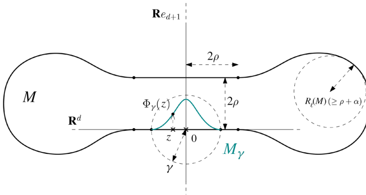
Fig. 4 The submanifolds M and M_\gamma used in the second part of the proof of the lower bound
