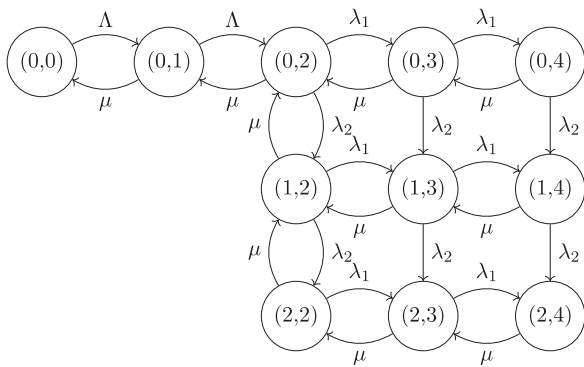
Fig. 15. Example Markov model C = 1, T = 2, N = 4, M = 2 .
