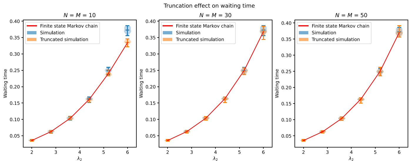
Fig. 3. Comparison of mean waiting time between values obtained from the Markov chain formula, values obtained from the truncated simulation and values obtained from the untruncated simulation.
