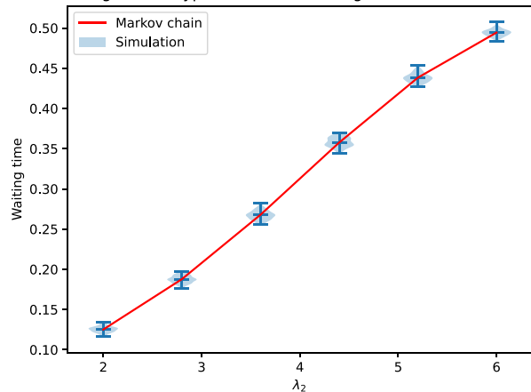
Fig. 18. Comparison of mean waiting time for type 2 individuals between values obtained from the Markov chain formulas and values obtained from simulation.
