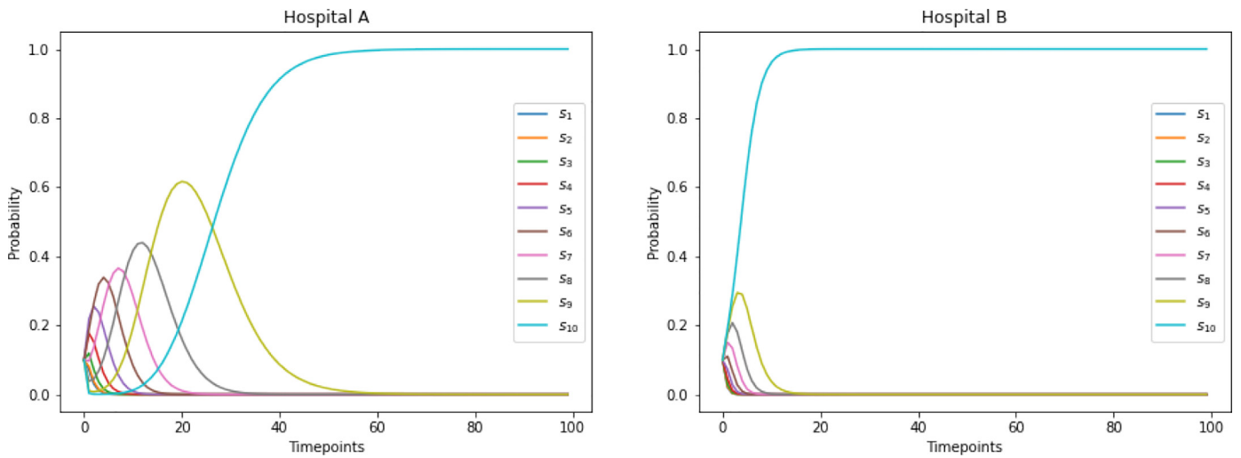
Fig. 8. Asymmetric replicator dynamics run.
