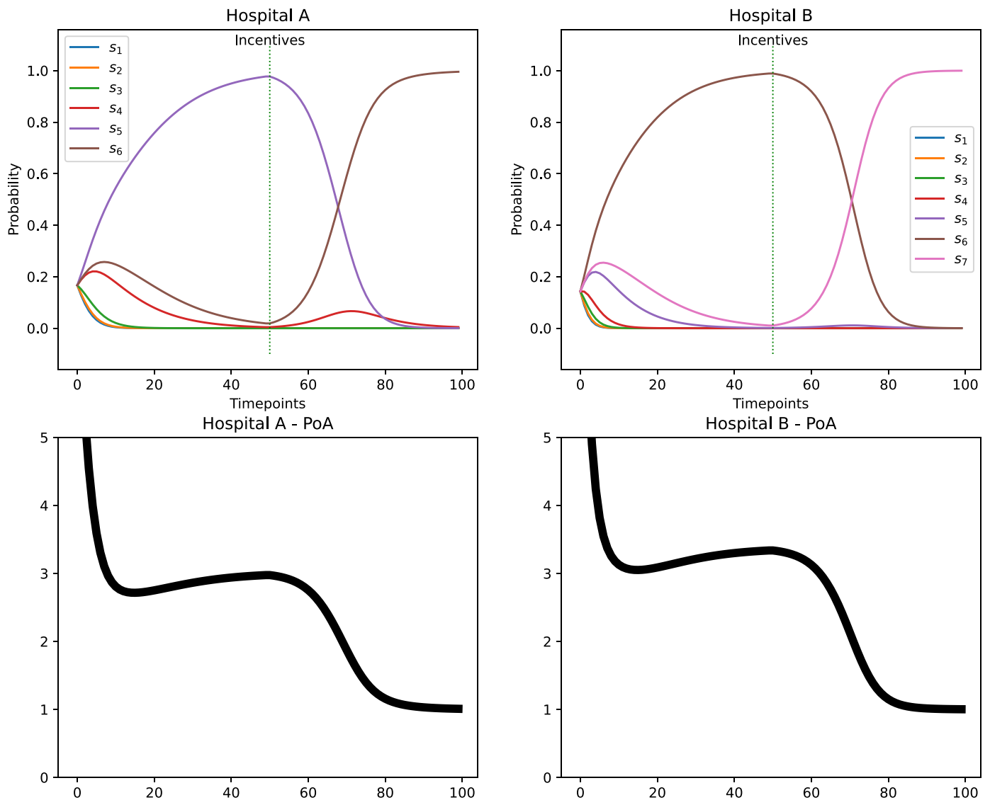
Fig. 12. The strategies played when running asymmetric replicator dynamics along with the compartmentalised price of anarchy of the blocking time at each iteration of the learning algorithm. After a number of iterations the most dominant strategy is being penalised.
