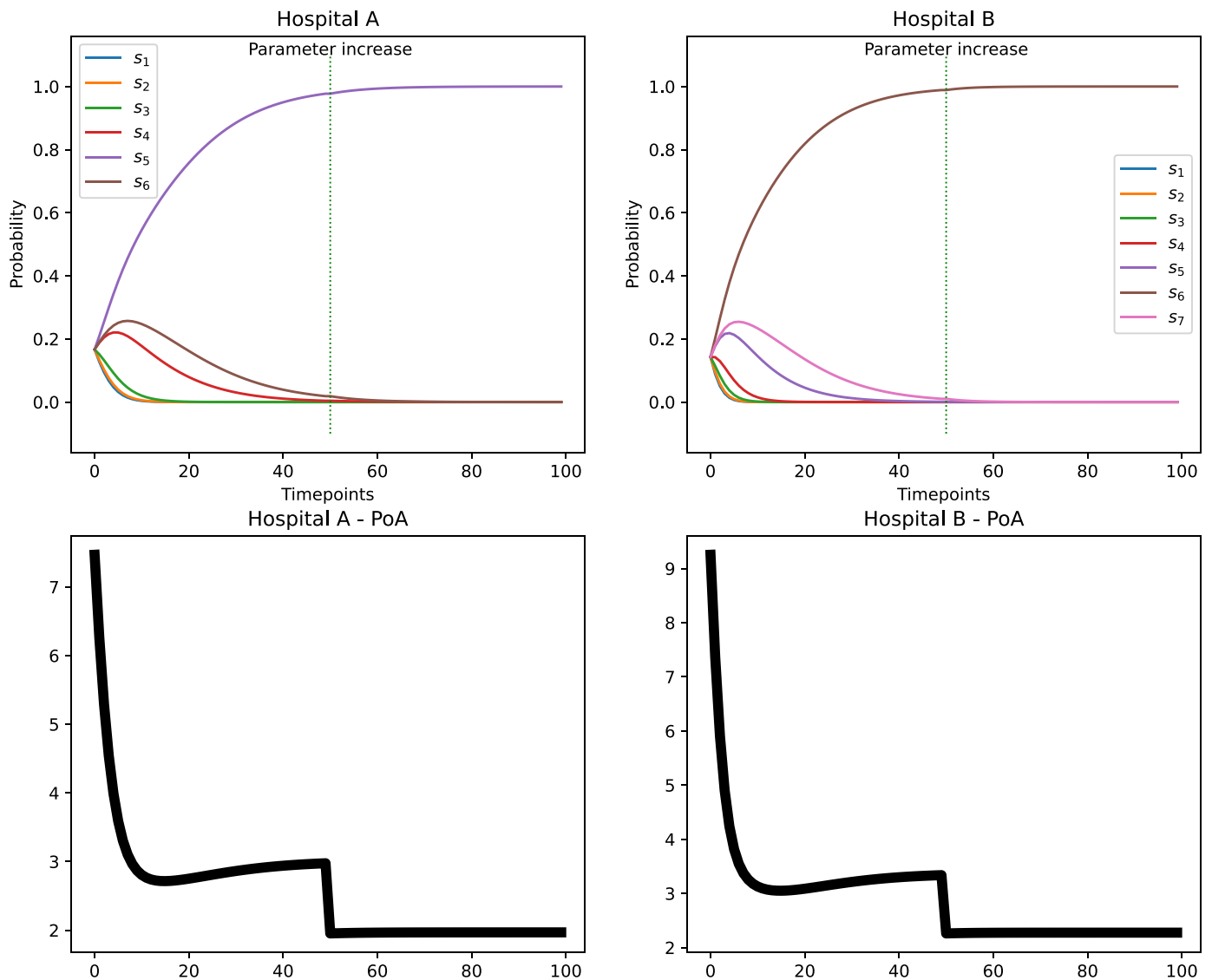
Fig. 11. The strategies played when running asymmetric replicator dynamics along with the compartmentalised price of anarchy of the blocking time at each iteration of the learning algorithm. After a number of iterations the number of servers for both systems are increased by one.
