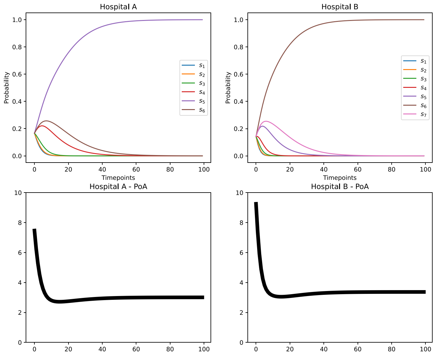
Fig. 9. The strategies played when running asymmetric replicator dynamics along with the compartmentalised price of anarchy of the blocking time at each iteration of the learning algorithm.
