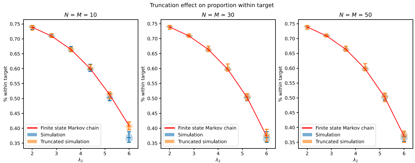
Fig. 5. Comparison of mean proportion of individuals within target time between values obtained from the Markov chain formula, values obtained from the truncated simulation and values obtained from the untruncated simulation.
