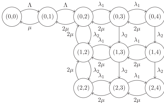
Fig. 16. Example Markov model C = 2, T = 2, N = 4, M = 2 .
