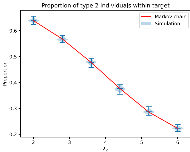
Fig. 20. Comparison of proportion within target time for type 2 individuals between values obtained from the Markov chain formulas and values obtained from simulation.
