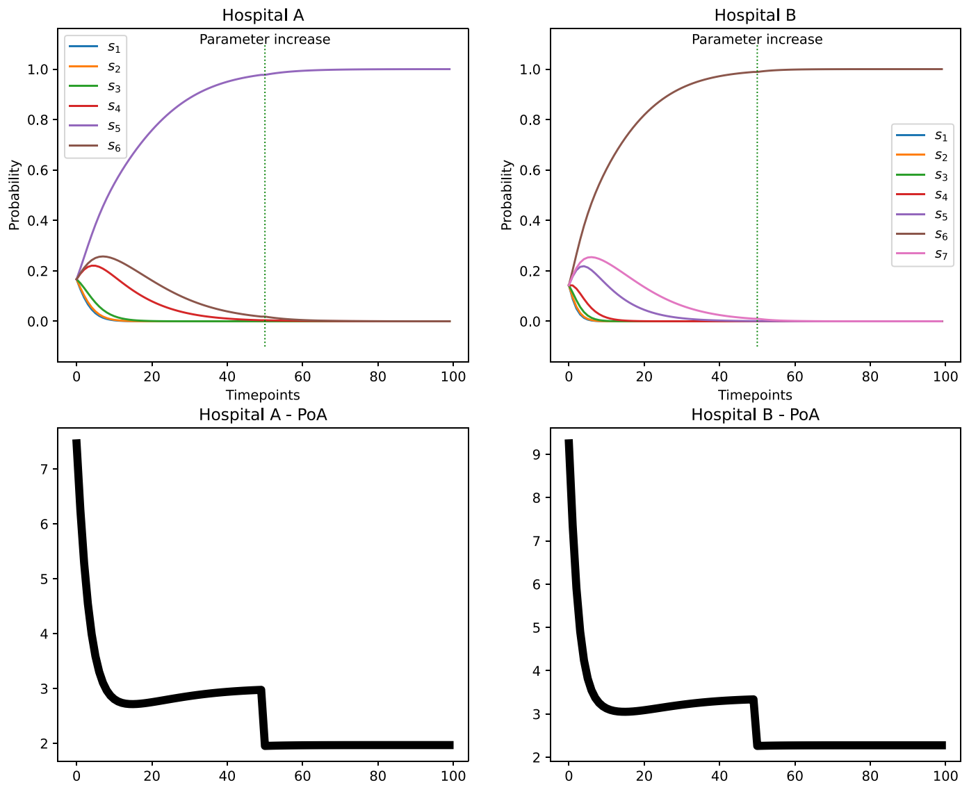
Fig. 10. The strategies played when running asymmetric replicator dynamics along with the compartmentalised price of anarchy of the blocking time at each iteration of the learning algorithm. After a number of iterations the arrival rate of ambulance patients is significantly increased to flood the system completely \lambda_2 = 24 .
