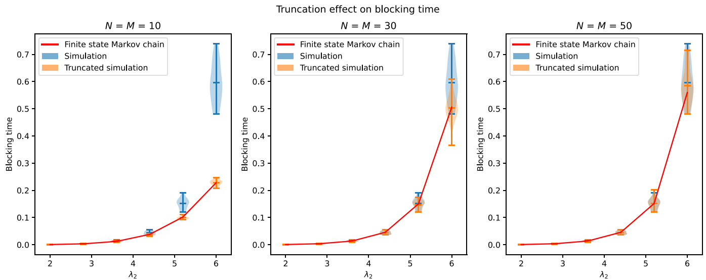
Fig. 4. Comparison of mean blocking time between values obtained from the Markov chain formula, values obtained from the truncated simulation and values obtained from the untruncated simulation.
