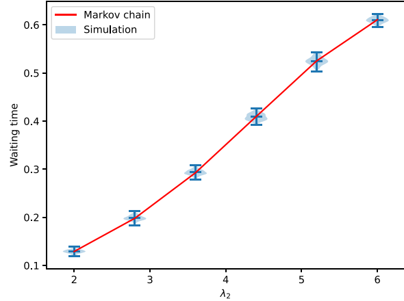
Fig. 17. Comparison of mean waiting time for type 1 individuals between values obtained from the Markov chain formulas and values obtained from simulation.
