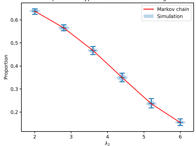
Fig. 19. Comparison of proportion within target time for type 1 individuals between values obtained from the Markov chain formulas and values obtained from simulation.
