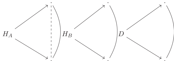
Fig. 7. Imperfect information Extensive Form Game between the distributor and the 2 queueing systems.
