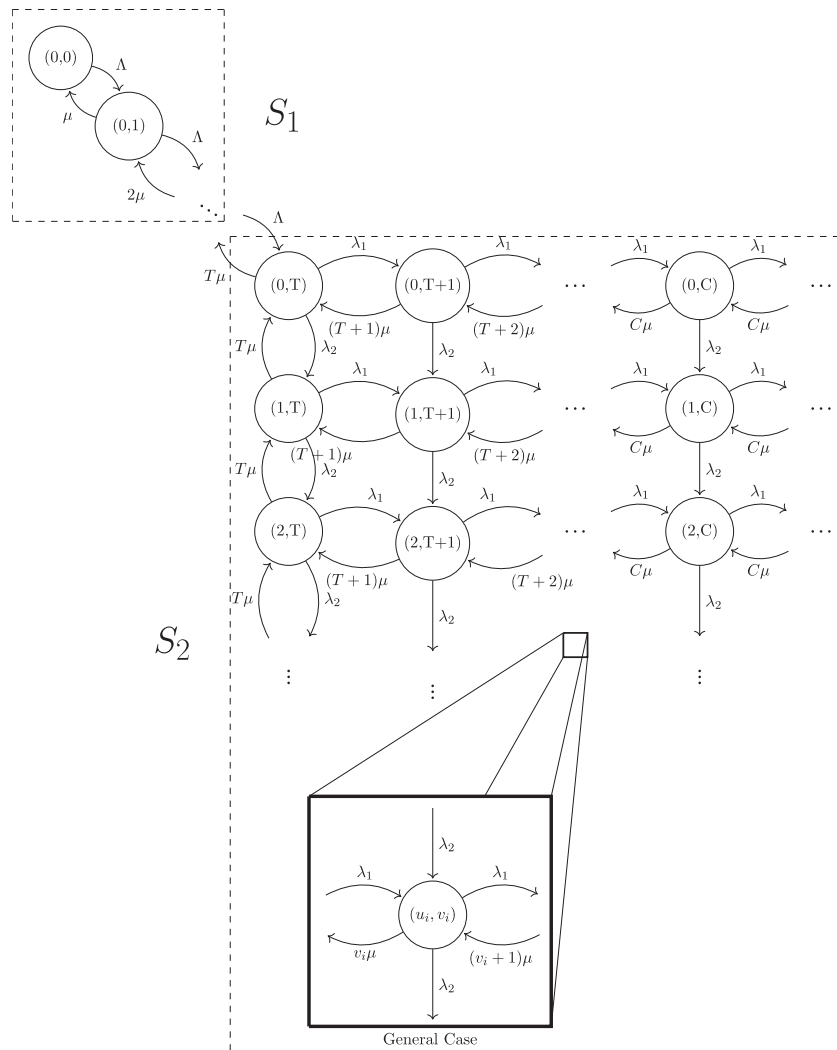
Fig. 2. General case of the Markov chain model.
