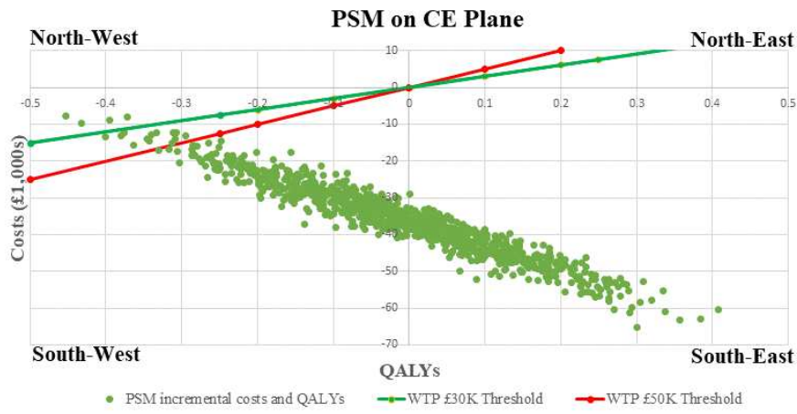
Figure 3. Partitioned Survival Model – incremental costs and QALYs on the cost-effectiveness plane. CE, cost-effectiveness; QALYs, quality-adjusted life years; WTP, willingness-to-pay.
