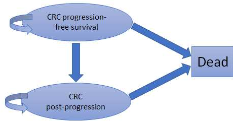
Figure 2. Markov Model. CRC, colorectal cancer.
