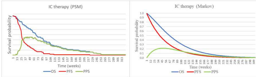
Figure 5. Comparison of PSM survival curves and Markov trace for IC therapy. IC, intermittent cetuximab; OS, overall survival; PFS, progression-free survival; PPS, post-progression survival.
