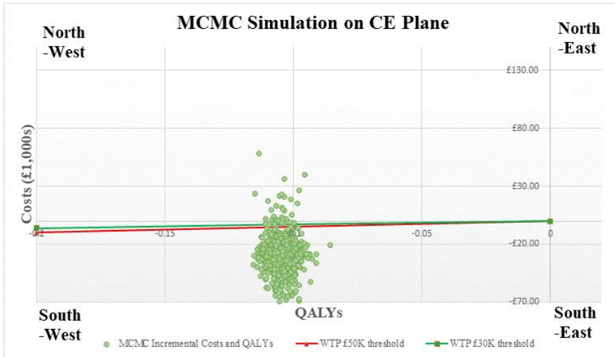
Figure 4. Markov Chain Monte Carlo simulation - incremental costs and QALYs on the cost-effectiveness plane. CE, cost-effectiveness; QALYs, quality-adjusted life years; WTP, willingness-to-pay.
