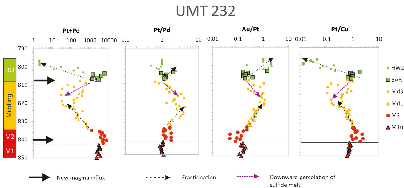
Fig. 5 Variation in PGE, Pt/Pd, Au/Pt and Pt/Cu in uppermost Flatreef, northern Bushveld lobe (data from Maier et al. 2021)
