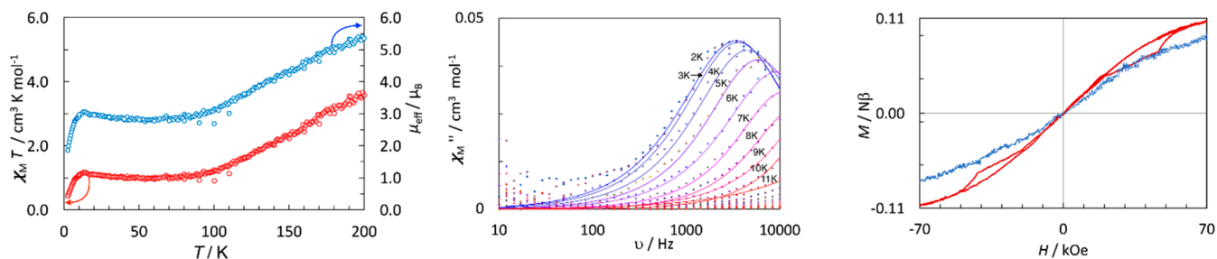
Figure 3. (left) Temperature dependences of \chi_M T and \mu_{\text{eff}} at T = 2.5\text{--}200 K in a field of 1 kOe. (center) Frequency dependence of \chi'' at the temperatures indicated in zero dc field. (right) Hysteresis at 2 K for the unrestrained (red) and restrained (blue) materials using an average sweep rate of 20 Oe \text{s}^{-1} .
