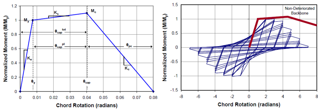
Fig. 5. Clough material implemented in OpenSees (Haselton et al., 2008)
