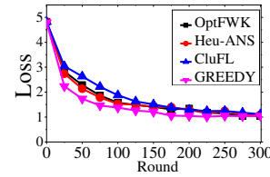
(b) The loss by changing the algorithms of each FL request.
