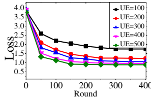
(b) The loss by varying the number UEs of each FL request.
