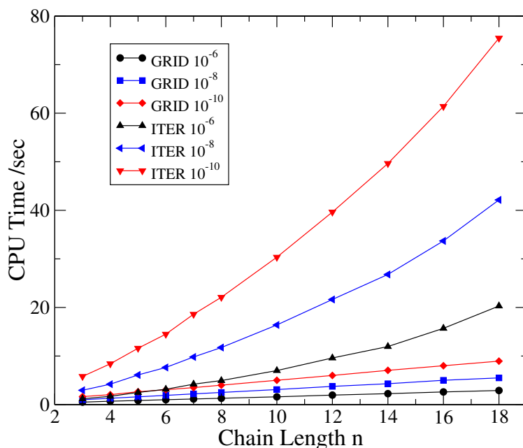
Figure 3. Computation times for linear alkanes C_nH_{n+2} (basis def2-TZVP, BLYP functional). Shown are the times for the adaptive grid generation (GRID) and the iteration time (ITER, 10 iterations) for 3 different values of T_{\text{grid}} . The calculations were run using a single core on a MacBook Pro laptop with M1 Max processor and 64 GB of memory.
