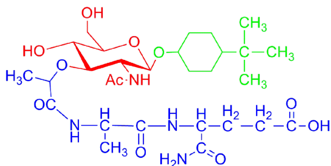
Scheme 1. Structure of MDP O -glycoside
