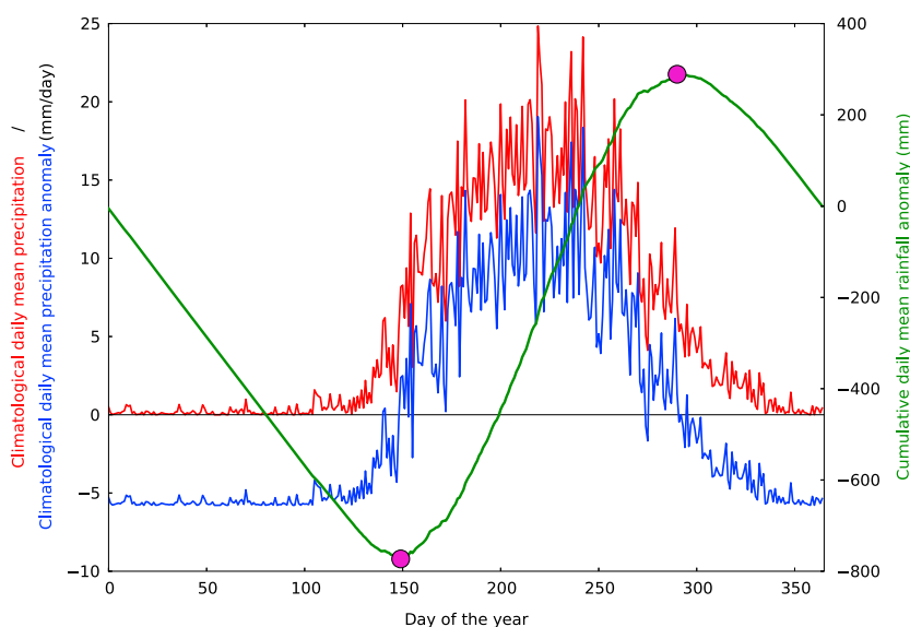
Figure 2. Climatological daily mean rainfall for each day of the year (red), climatological daily mean rainfall anomaly (blue), and climatological cumulative daily mean rainfall anomaly (green) for 9.5°N, 14.5°W from GPCP averaged over 1997–2014. The magenta dots mark the extent of the climatological water season.
