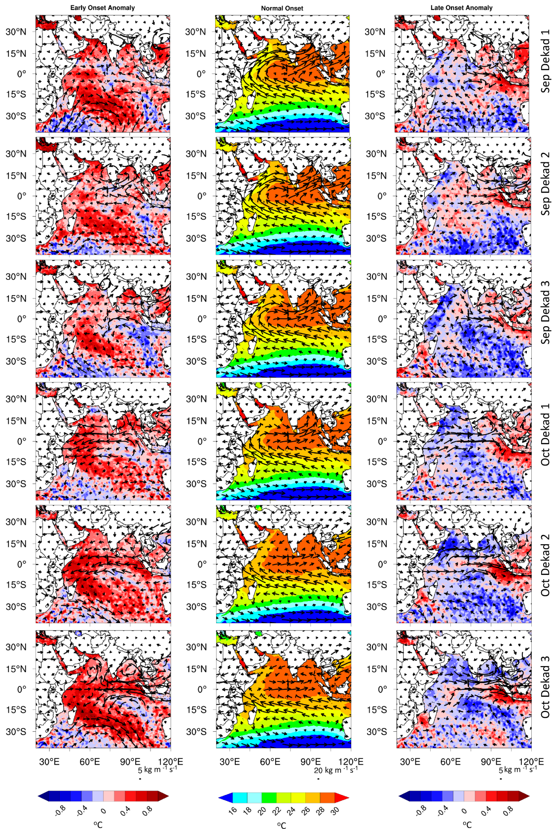
FIGURE 7 Vertically integrated moisture flux (vectors, kg m -1 s -1 ) and sea surface temperatures (shaded, °C) composites for the early onset anomaly (left column), mean onset (middle column) and late onset anomaly (right column) over Eastern Africa, from Dekad 1 of September (top row) to Dekad 3 of October (bottom row)
