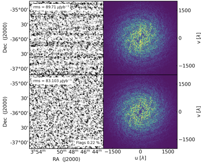
Fig. 6. HI data before (top) and after (bottom) flagging the broad-band RFI near u = 0 for a typical MeerKAT 5 h observation. The top row shows broad horizontal stripes in the image plane (left) and a corresponding bright vertical stripe at u = 0 in its Fourier transform (right). The bottom row shows that, in this case, by flagging just 0.22% of the data (as indicated in the bottom right corner of the left panel), the stripes are no longer visible and the formal noise of the image decreases by 8% (see the noise values reported in the top left corner of the left panels). After flagging, the bright vertical stripe is no longer visible in the Fourier transform of the image (bottom right panel). We note that this figure shows the image (and its Fourier transform) that is obtained by combining all science scans of a 5 h observation, whereas the flags are calculated for each scan independently (see Sect. 3.6).
