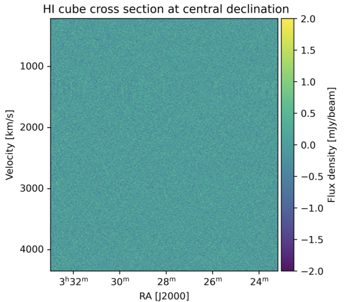
Fig. 7. Two slices through the 24'' tapered HI cube made for a typical MeerKAT 5 h observation. These slices show no artefacts due to residual RFI or continuum subtraction errors. Typically, the RA-velocity slices show some faint vertical structure in channel ranges that are excluded from the visibility spectral fit described in Sect. 3.5 (in this case, \sim 1200\text{--}1500 \text{ km s}^{-1} ).
