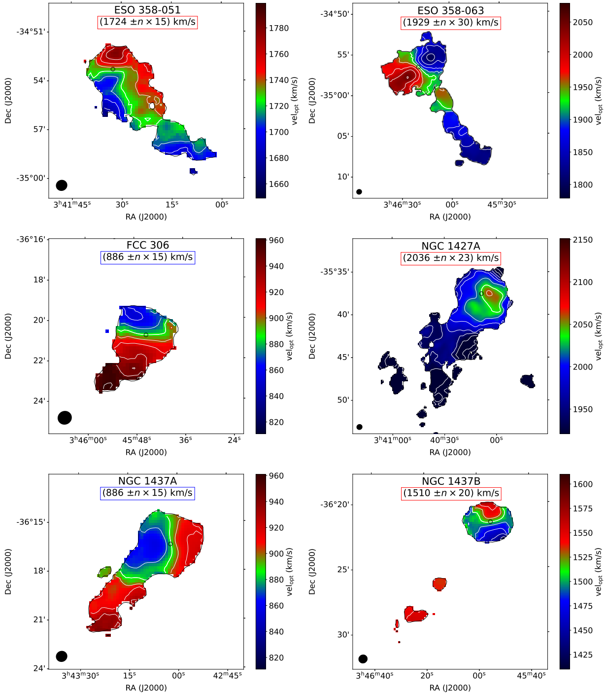
Fig. 10. Moment-1 HI velocity field of the six galaxies with a one-sided HI tail. The galaxy name is given at the top of each image. Below the galaxy name, we indicate the HI systemic velocity, which is represented by the thick white iso-velocity contour in the figure, as well as the levels of the other contours ( n = 0, 1, \dots ). The coloured frame around the contour levels indicates whether a galaxy is blue- or redshifted relative to NGC 1399, whose velocity is \sim 1425 \text{ km s}^{-1} . The bottom left black ellipse represents the 41'' HI resolution. The small open black circle represents the galaxy centre. The thin black contour is the first HI contour shown in Fig. 9.
