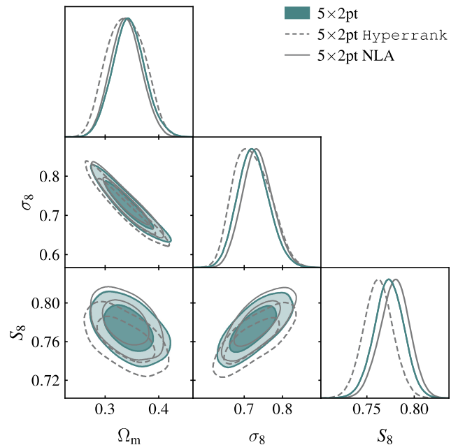
FIG. 15. Parameter constraints obtained when using alternative prescriptions for modeling photometric redshift biases and intrinsic alignments. The teal curves show our baseline results, while the grey dashed curves show results assuming the HYPERRANK method for calibrating the source galaxy redshift distributions, and the grey solid curves show results assuming the NLA intrinsic alignment model (rather than the baseline TATT model). In both cases, there are minimal shifts relative to our baseline results.
