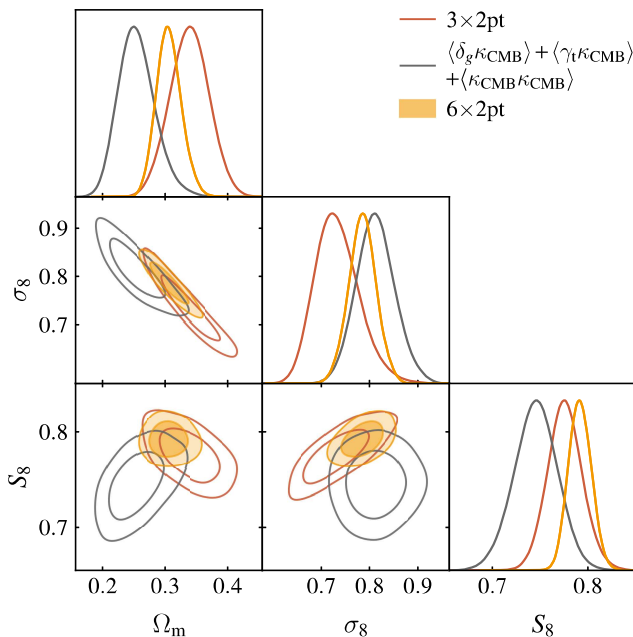
FIG. 5. Comparison of constraints on \Lambda CDM from 3 \times 2 pt (red) with the constraints from the other probes of 6 \times 2 pt, i.e. \langle \delta_g \kappa_{\text{CMB}} \rangle + \langle \gamma_t \kappa_{\text{CMB}} \rangle + \langle \kappa_{\text{CMB}} \kappa_{\text{CMB}} \rangle (grey). The joint analysis of both ( 6 \times 2 pt) is shown in orange. The two subsets of the full 6 \times 2 pt analysis are in reasonable agreement. The 6 \times 2 pt analysis prefers higher S_8 than either of the two subsets.
