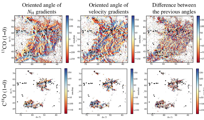
Fig. D.5. Maps of oriented angles of the gradients of the column density and centroid velocity gradients for the low-velocity layer of the Orion B9 area. The figure layout is identical to Fig. D.2
