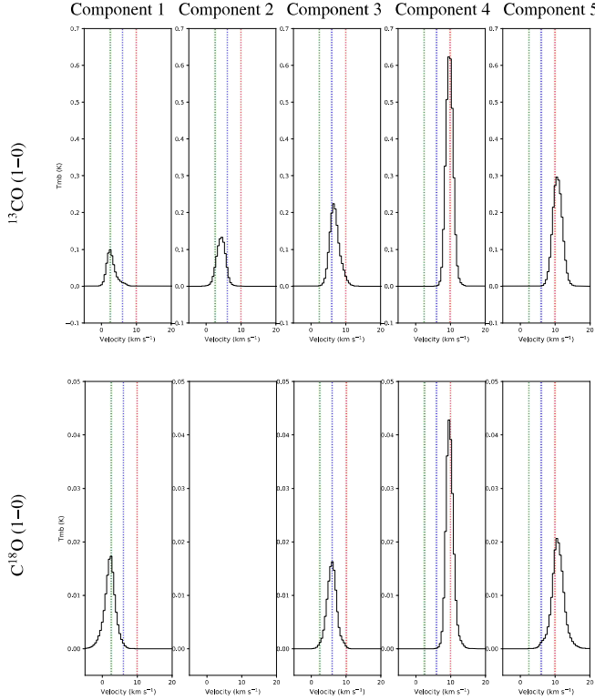
Fig. B.1. Mean spectrum of each Gaussian component fit by ROHSA for the ^{13}\text{CO} (1–0) (top) and \text{C}^{18}\text{O} (1–0) (bottom) line. The color dotted lines show the systemic velocity of the three cloud layers.
