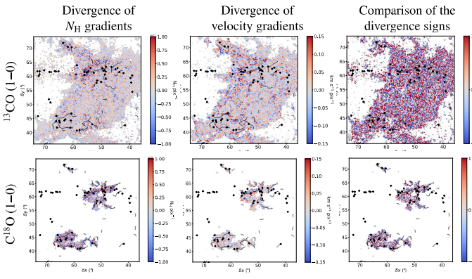
Fig. D.6. Divergence maps for the low-velocity layer of the Orion B9 area. The figure layout is identical to Fig. D.2
