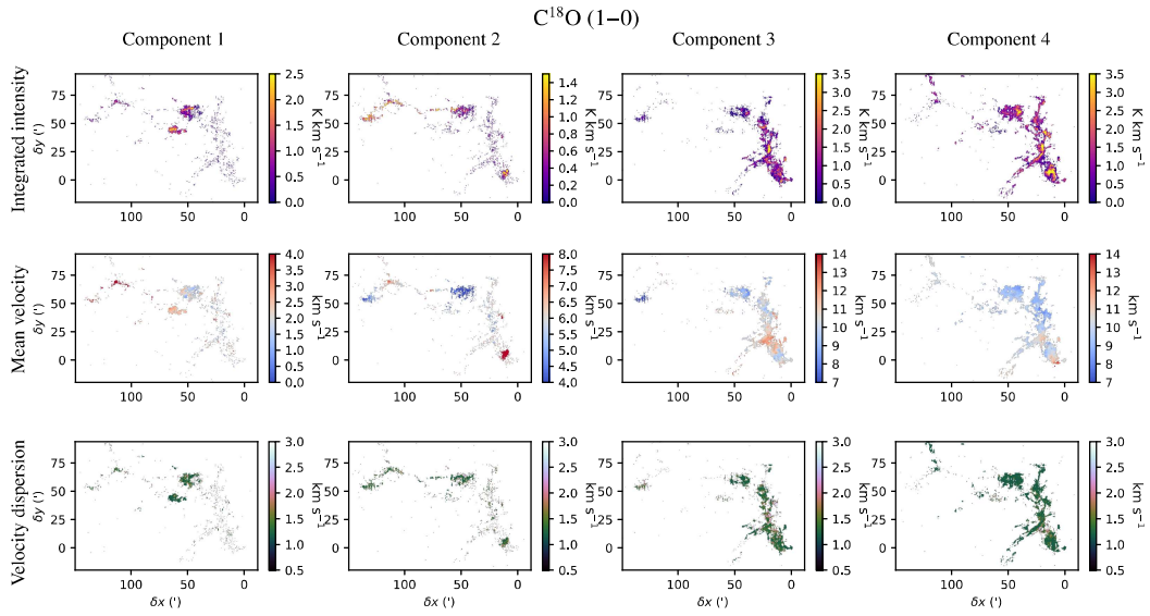
Fig. B.2. Zero-order (integrated intensity, top), first-order (mean velocity, middle), and second-order (velocity dispersion, bottom) moment maps of each of the four Gaussian components fit by ROHSA for the \text{C}^{18}\text{O} (1–0) line. Isolated pixels and pixels with a signal-to-noise ratio lower than 3 are blanked.
