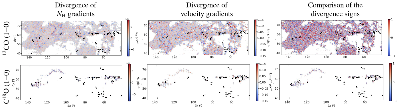
Fig. D.3. Divergence maps of the column density gradients in \text{N}_{\text{H}} \text{ pix}^{-1} (left) and the velocity gradients in \text{km s}^{-1} \text{ pix}^{-1} (middle) for the intermediate-velocity layer of the Cloak area from the ^{13}\text{CO} (1-0) (top) and the \text{C}^{18}\text{O} (1-0) (bottom) emission. Right: comparison maps of the sign between the velocity gradient divergence and the column density gradient divergence. The values -1 (blue) or 1 (red) show the pixels where velocity and column density gradients both converge or both diverge. The value 0 (gray) indicates regions where the sign of at least one gradient is ill-defined because its modulus is close to zero. The black lines show the filamentary structure and the diamond dots show the dense cores identified by the Herschel Gould Belt Survey (Könyves et al. 2020).
