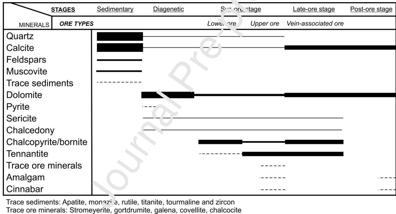
Fig. 12. Paragenetic sequence of the Gortdrum Cu-Ag deposit.
